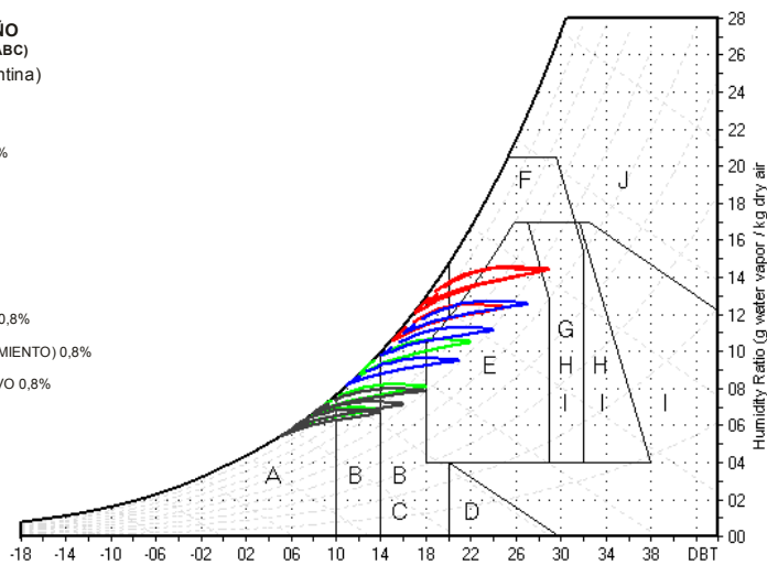
ABC 1.3 - Bioclimatic Chart for pressure of 101.325 kPa (Elev: 0 m)
