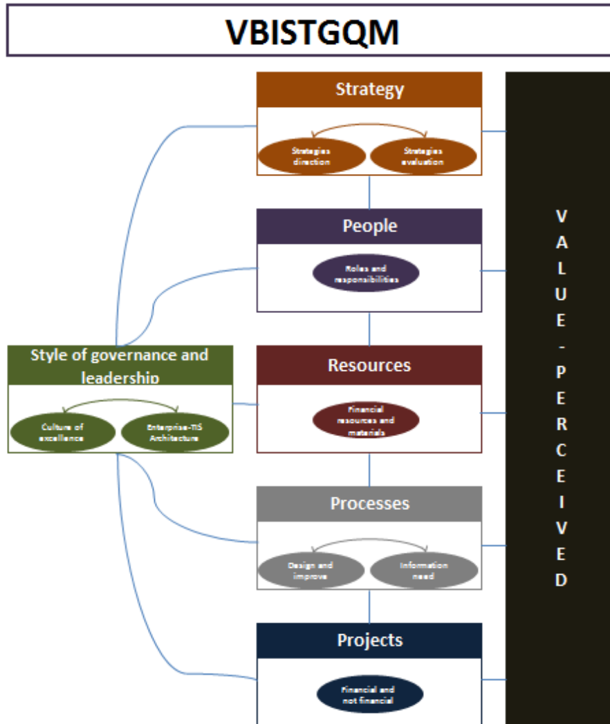
Figure 1. VBISTGQM model
