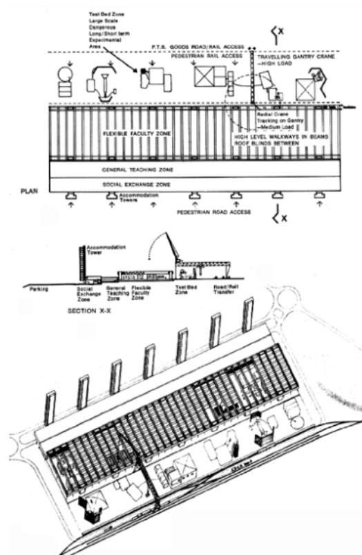
Fig. 26. Cedric Price, complejo Potteries Think belt, 1971. Architectural Design , 1966, October.
