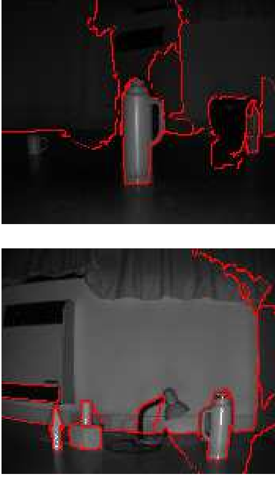
Figure 3: Segmentation obtained using the proposed method
