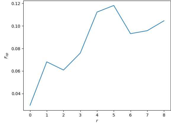
Figure 2: Influence of parameter r in relation to the precision and recall metrics of objects and parts.
