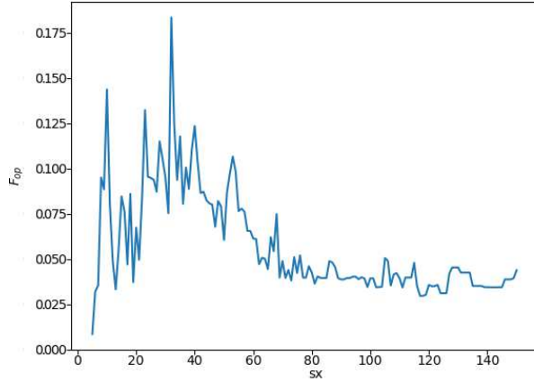
Figure 1: Influence of parameter s_x in relation to the precision and recall metrics of objects and parts.
