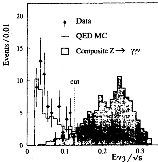
Fig. 2. The energy distribution for least energetic photon, the prediction from QED and the prediction [2,3] for a composite Z decaying directly into \gamma\gamma (arbitrarily normalized).
