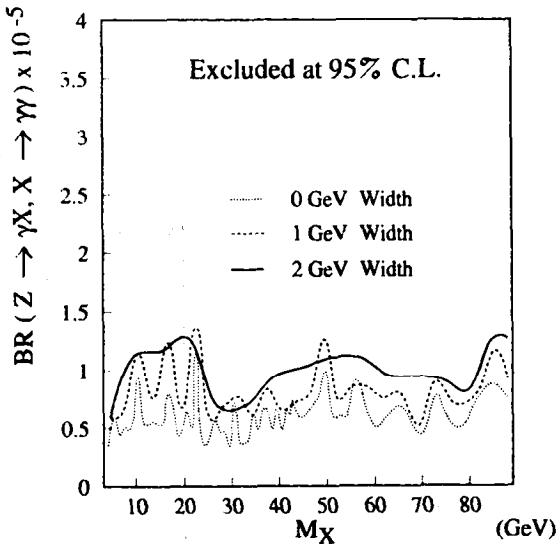
Fig. 4. The upper limit on BR(Z \rightarrow \gamma X, X \rightarrow \gamma\gamma) as a function of M_X . The scalar particle X is assumed to have a mass distribution which is either a delta-function or a Breit-Wigner with a width of 1 or 2 GeV, produced with a (1 + \cos^2\theta) polar angle distribution.
