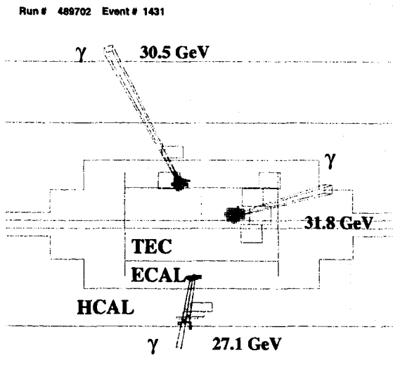
Fig. 1. A display of a \gamma\gamma\gamma event in the inner L3 detector, shown along the beam axis. The photon energies are indicated.
