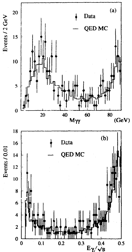
Fig. 3. (a): The \gamma\gamma invariant mass spectra for the observed \gamma\gamma events (three entries/event) with E_\gamma > 2 GeV and the prediction from QED. (b): The photon energy spectrum (three entries/event) for the observed \gamma\gamma events; and the prediction from QED.
