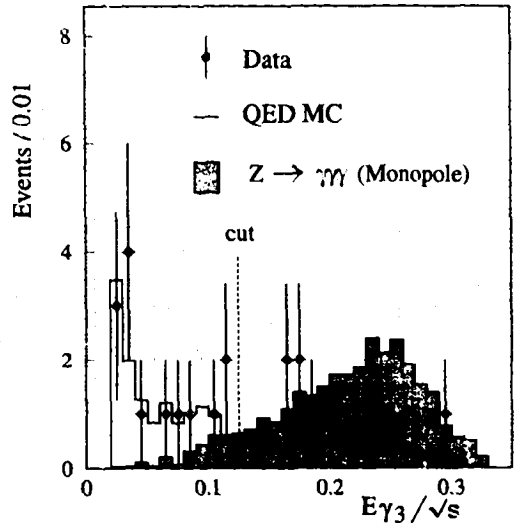
Fig. 5. The energy distribution for the least energetic photon in \gamma\gamma\gamma events for \gamma 's in the central detector region ( |\cos\theta_\gamma| < 0.75 ), the prediction from QED and the prediction (arbitrarily normalized) from the monopole model [4].
