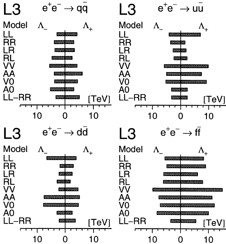
Fig. 2. One-sided 95% confidence level lower limits on the scales \Lambda_+ and \Lambda_- for contact interactions in hadronic channels and in all channels combined. The limits correspond to the values given in Table 3.
