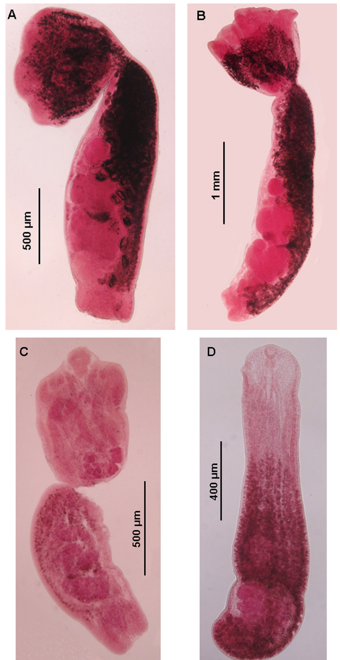
Figure 1. Trematoda of strigiform birds from Central and North-eastern Argentina. A: Strigea falconis brasiliensis from Asio clamator . B: Strigea magniova from Tyto alba . C: Australapatemon magnacetabulum from Asio clamator . D: Neodiplostomum travassosi
