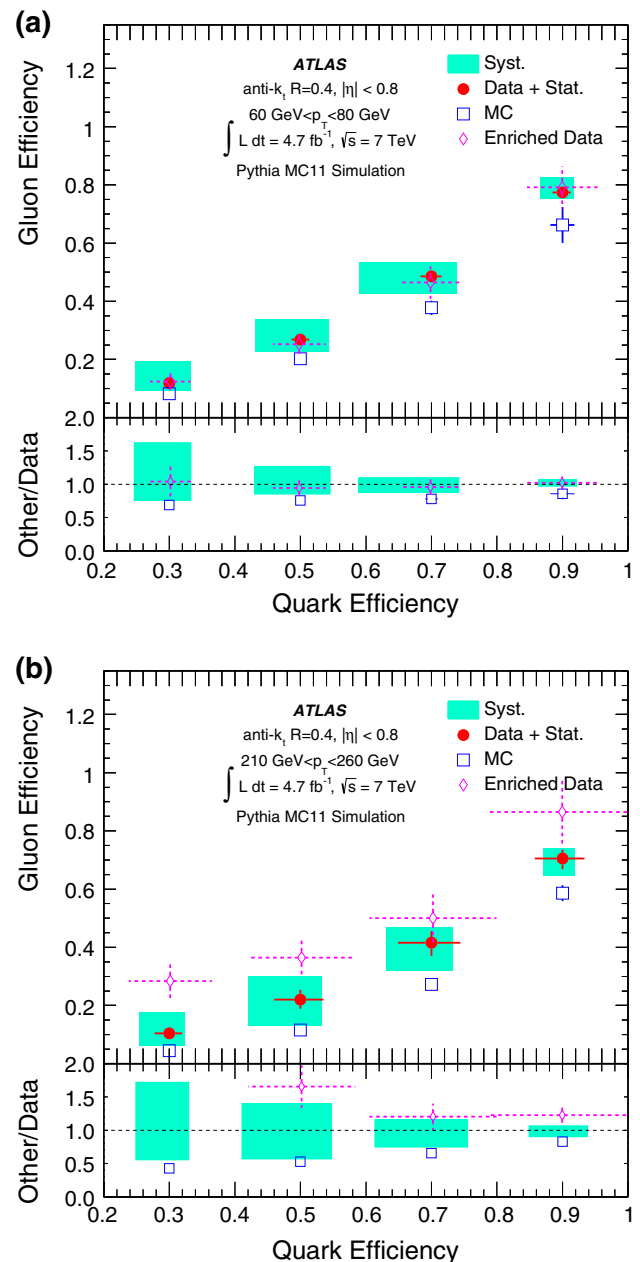
Fig. 6 Gluon-jet efficiency as a function of quark-jet efficiency as calculated using jet properties extracted from data ( solid symbols ), purified in data through kinematic cuts ( empty diamonds ), and extracted from PYTHIA 6 MC simulation ( empty squares ). Jets with a 60 < p_T < 80 GeV and b 210 < p_T < 260 GeV and |\eta| < 0.8 are reconstructed with the anti- k_r algorithm with R = 0.4 . The shaded band shows the total systematic uncertainty on the data. The bottom of the plot shows the ratio of PYTHIA 6 MC simulation or the enriched data samples to the extracted data. The error bands on the performance in the data are drawn around 1.0
