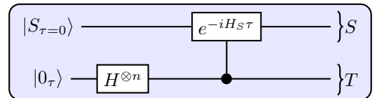
FIG. 1. Schematic circuit representing the generation of the history state (14) in the special time basis, where the system evolves according to a constant Hamiltonian H_S . Here H^{\otimes n} denotes the Hadamard operator over n qubits, with 2^n = N .
