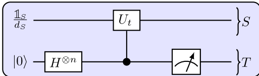
FIG. 4. (Color online) Schematic circuit representing the measurement of the operator overlaps (79).
