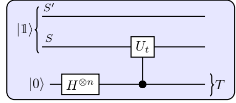
FIG. 3. (Color online) Schematic circuit representing the generation of the operator history state (60).
