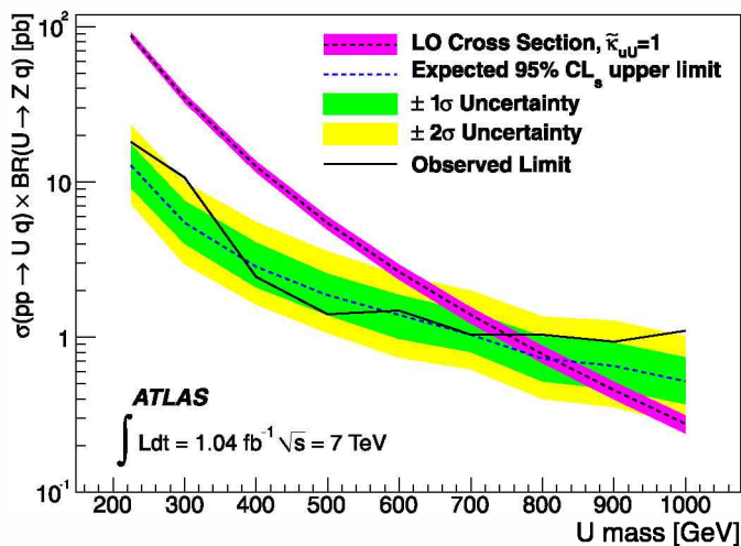
Fig. 3. Upper limits at 95% confidence level on the cross section times branching ratio \sigma(pp \rightarrow Qq) \times \text{BR}(Q \rightarrow Vq) for the CC (top) and NC (bottom) channels as a function of mass. The leading-order (LO) theoretical cross section assumes \tilde{\kappa}_{uD} = 1 and \tilde{\kappa}_{uU} = 1 on the top and bottom, respectively. The width of the dark band around it corresponds to the theoretical uncertainty described in the text. The expected cross section upper limit is determined by the median result of background-only pseudoexperiments, and is shown with its 1\sigma and 2\sigma uncertainties, respectively.
