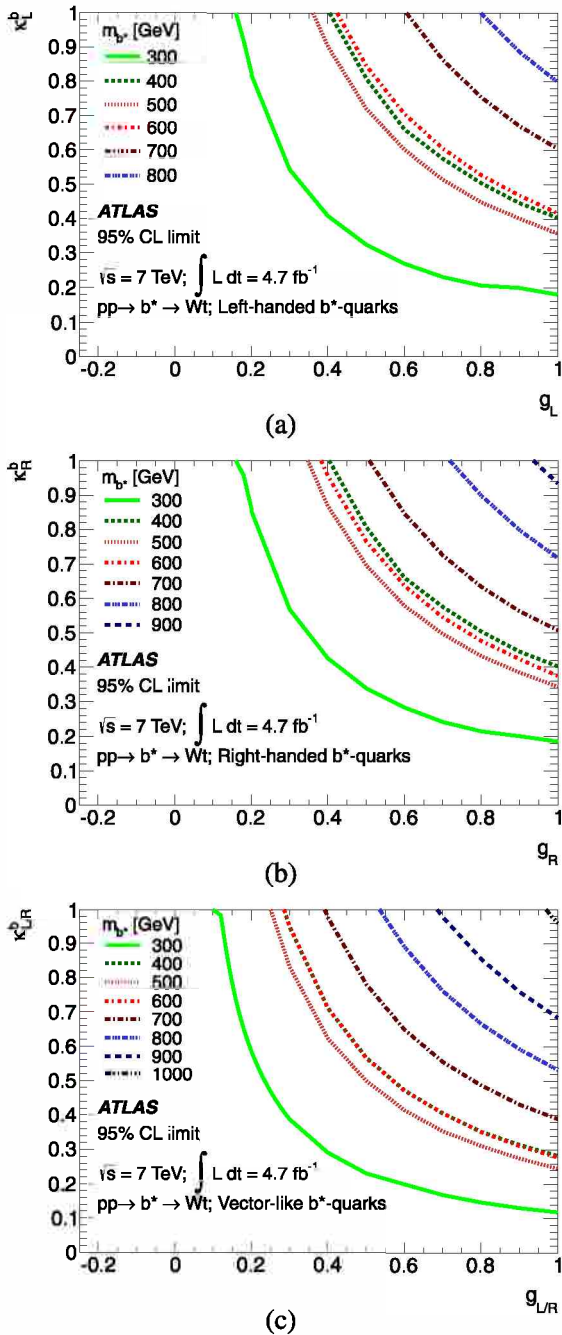
Fig. 7. Limit contours at the 95% CL as a function of the coupling parameters for several different b^* -quark masses, for (a) left-handed b^* quarks, (b) right-handed b^* quarks and (c) vector-like b^* quarks.
