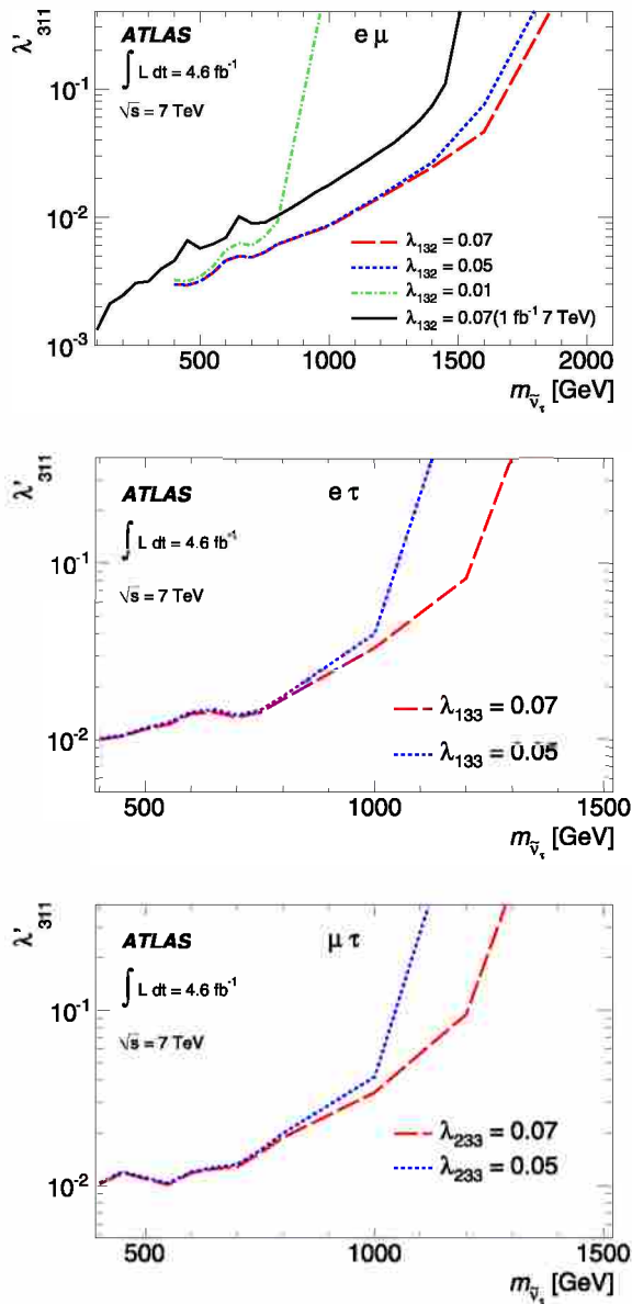
Fig. 3. The 95% CL limits on \lambda'_{311} as a function of sneutrino mass for assumed values of \lambda_{13k} for the e\mu (top), e\tau (middle), and \mu\tau (bottom) modes. For the e\mu mode, the black solid curve is the previous ATLAS result based on 1\text{ fb}^{-1} of data at 7 TeV.
