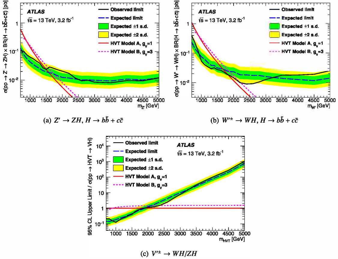
Fig. 3. Upper limits at the 95% CL for (a) the production cross-section of Z' times its branching fraction to ZH and the branching fraction sum BR(H \rightarrow b\bar{b} + c\bar{c}) and (b) the production cross-section of W' times its branching fraction to WH and the branching fraction sum BR(H \rightarrow b\bar{b} + c\bar{c}) . Upper limits at the 95% CL for (c) the scaling factor of the production cross-section for V' times its branching fraction to WH/ZH in Model A. The production cross-sections predicted by Model A and Model B are shown for comparison. In all cases H \rightarrow b\bar{b} and H \rightarrow c\bar{c} decays are included at the branching fractions predicted in the SM.
