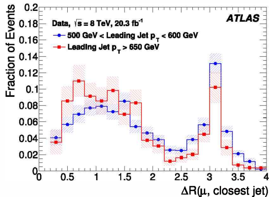
Fig. 4. Unfolded distribution from background-subtracted data of the angular separation between the muon and the closest jet for events with 500 \text{ GeV} < p_{\text{T}}^{\text{leading jet}} < 600 \text{ GeV} (blue circles) and p_{\text{T}}^{\text{leading jet}} > 650 \text{ GeV} (red squares) from the signal region. Distributions are normalised to unity. The shaded error band on the unfolded measurement corresponds to the sum of the statistical and systematic uncertainties. (For interpretation of the references to colour in this figure legend, the reader is referred to the web version of this article.)
