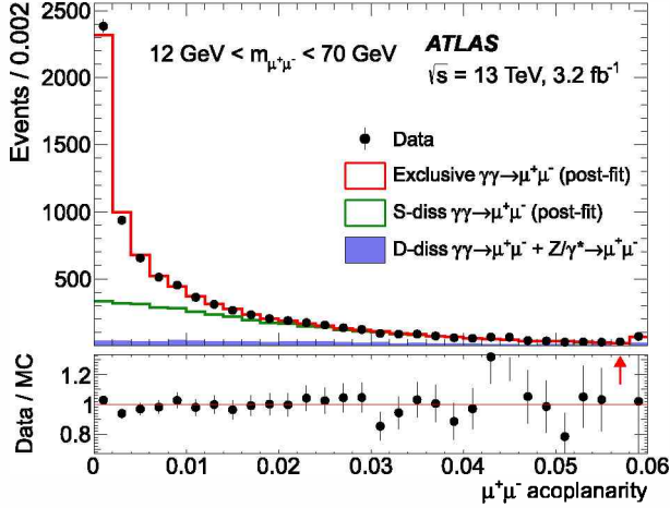
Fig. 3. Dimuon acoplanarity distribution after signal selection requirements. Data are shown as points with statistical error bars, while the histograms, in top-to-bottom order, represent the simulated exclusive signal, the S-diss and the sum of D-diss and DY backgrounds. The exclusive and S-diss yields are determined from the fit described in the text. The last bin includes overflow events. The lower panel indicates the ratio of data to the predicted distribution. Red arrow indicates a bin where the corresponding entry falls outside the plotted range. (For interpretation of the references to colour in this figure legend, the reader is referred to the web version of this article.)
