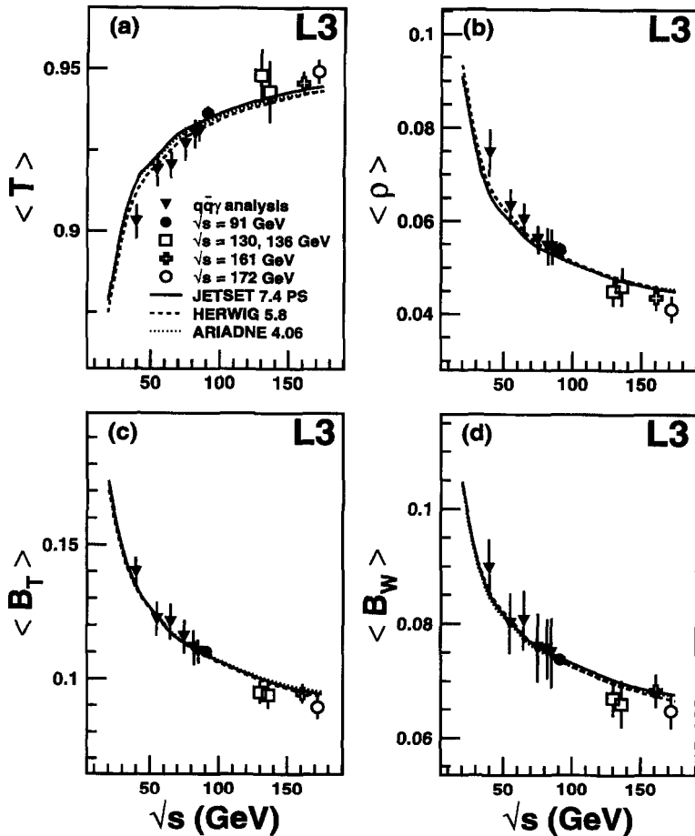
Fig. 3. Distributions for the mean values of (a) thrust ( T ), (b) scaled heavy jet mass ( \rho ), (c) total jet broadening ( B_T ), and (d) wide jet broadening ( B_W ) as a function of centre-of-mass energy. The results of the analysis presented here are compared with our measurements at and above the Z peak. The lines correspond to the predictions of various QCD models.
