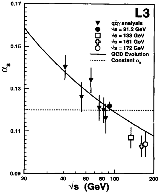
Fig. 5. Measured values of \alpha_s from the event shape distributions as a function of centre-of-mass energy. The errors correspond to the experimental uncertainties only. The solid and dashed lines are fits with the energy dependence of \alpha_s as given by QCD and with a constant \alpha_s , respectively.
