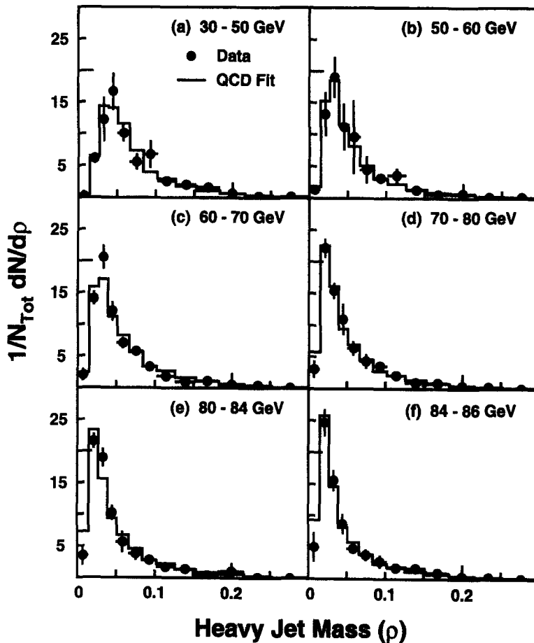
Fig. 4. Corrected scaled heavy jet mass ( \rho ) distributions at different reduced centre-of-mass energies (a-f). The histograms are the fitted QCD distributions.
