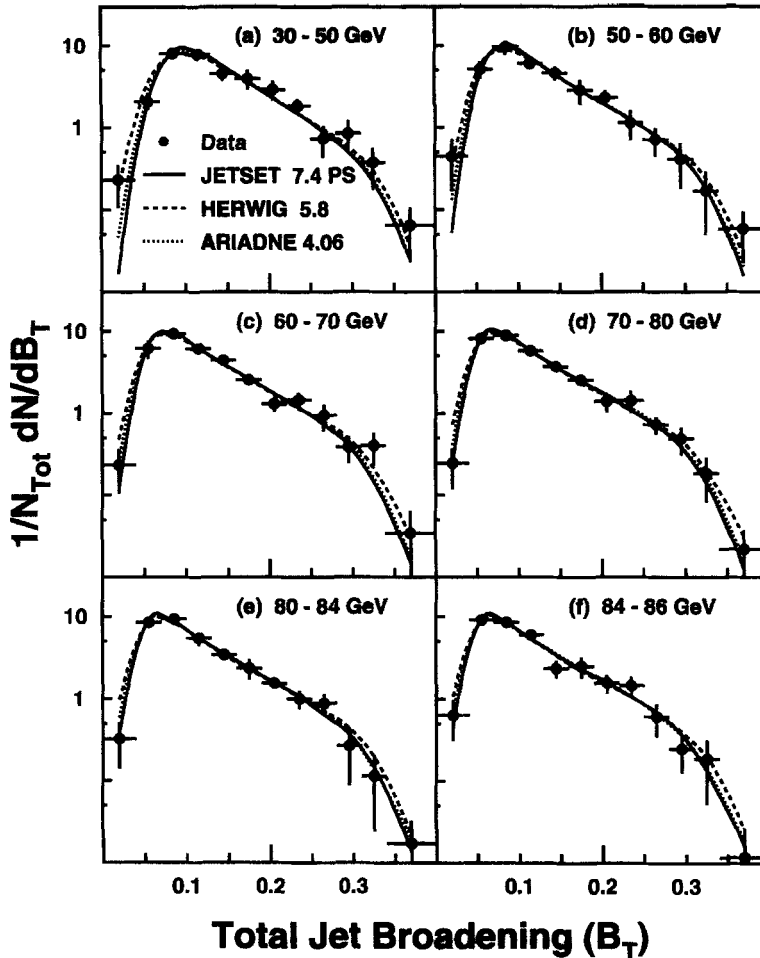
Fig. 2. Corrected total jet broadening distributions at different reduced centre-of-mass energies (a-f). The lines correspond to the predictions of different QCD models.
