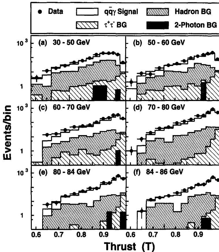
Fig. 1. Measured thrust distributions at different reduced centre-of-mass energies (a-f). The solid lines correspond to the overall expectations from theory. The shaded areas refer to different backgrounds and the open area refers to the signal predicted by JETSET. Note that the histograms have a variable bin width.
