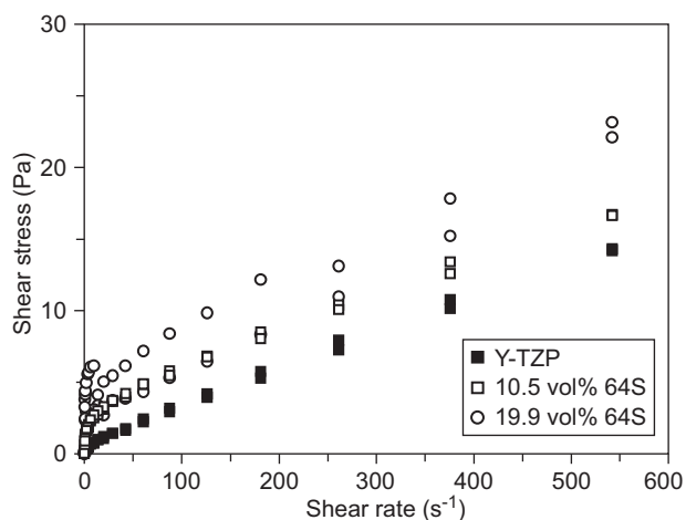
Figure 9. Flow curves of shear stress versus shear rate for 43 vol% slips with the optimum amount of \text{NH}_4\text{PA} solution added at \text{pH}\approx 9 .
