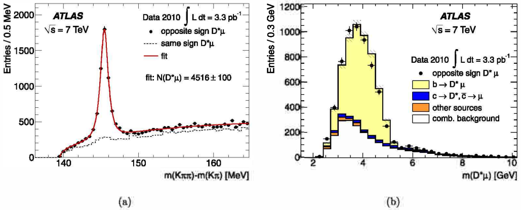
Fig. 1. (a) Distribution of the mass difference \Delta m for D^{*+}\mu^{-} combinations of opposite charge (points) and same charge (dashed line). The solid line shows the result of the fit described in the text. (b) Distribution of the opposite charge D^{*+}\mu^{-} invariant mass, for mass combinations within \pm 3\sigma of the \Delta m peak, without applying the invariant mass cut described in the text. The measured distribution is compared with the MC simulation, including the contribution of different sources of signal. The hashed bands show the MC statistical uncertainty.
