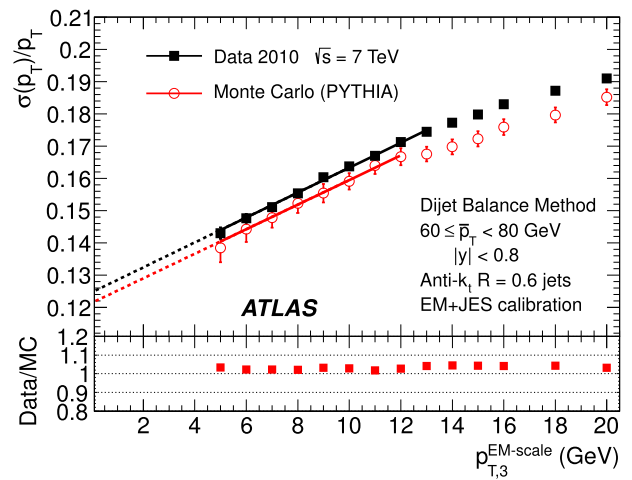
Fig. 2 Fractional jet p_T resolutions, from Eq. (2), measured in events with 60 \leq \bar{p}_T < 80 GeV and with third jet with p_T less than p_{T,3}^{EM-scale} , as a function of p_{T,3}^{EM-scale} , for data (squares) and Monte Carlo simulation (circles). The solid lines correspond to linear fits while the dashed lines show the extrapolations to p_{T,3}^{EM-scale} = 0 . The lower panel shows the ratio between data and MC simulation. The errors shown are only statistical
