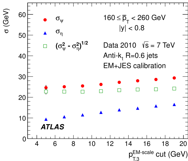
Fig. 7 Standard deviations \sigma_{\psi}^{\text{calo}} , \sigma_{\eta}^{\text{calo}} and [(\sigma_{\psi}^2 - \sigma_{\eta}^2)^{\text{calo}}]^{1/2} as a function of the upper p_{T,3}^{\text{EM-scale}} cut, for R = 0.6 anti- k_t jets with 160 \leq \bar{p}_T < 260 GeV. The errors shown are only statistical
