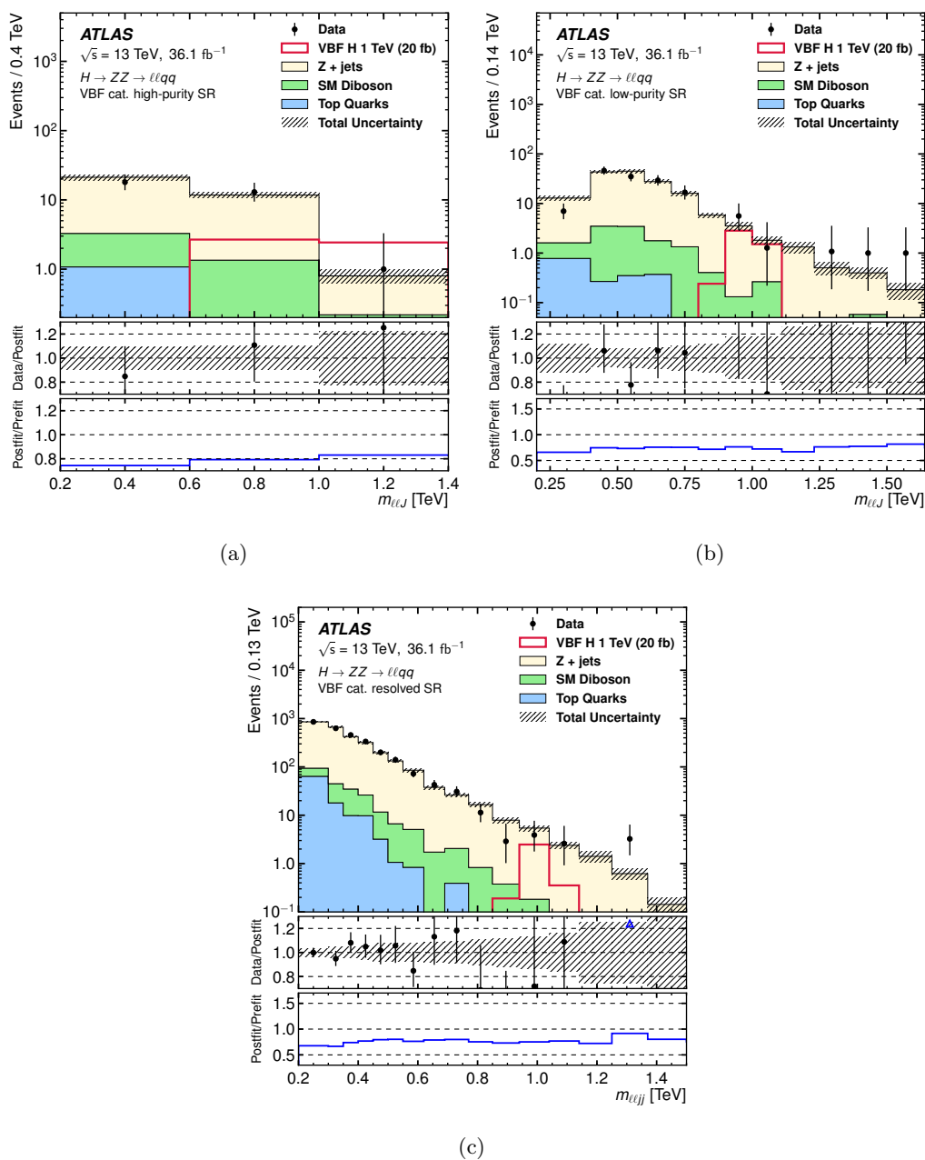
Figure 7. Comparisons of the observed data and expected background distributions of the final discriminants of the VBF category for the H \rightarrow ZZ \rightarrow \ell\ell qq search: m_{\ell\ell J} of (a) high-purity and (b) low-purity signal regions; (c) m_{\ell\ell jj} of the resolved signal region. For illustration, expected distributions from the VBF production of a 1 TeV Higgs boson with \sigma \times \mathcal{B}(H \rightarrow ZZ) = 20 fb are also shown. The middle panes show the ratios of the observed data to the background predictions. The uncertainty in the total background prediction, shown as bands, combines statistical and systematic contributions. The blue triangles in the middle panes indicate bins where the ratio is nonzero and outside the vertical range of the plot. The bottom panes show the ratios of the post-fit and pre-fit background predictions.
