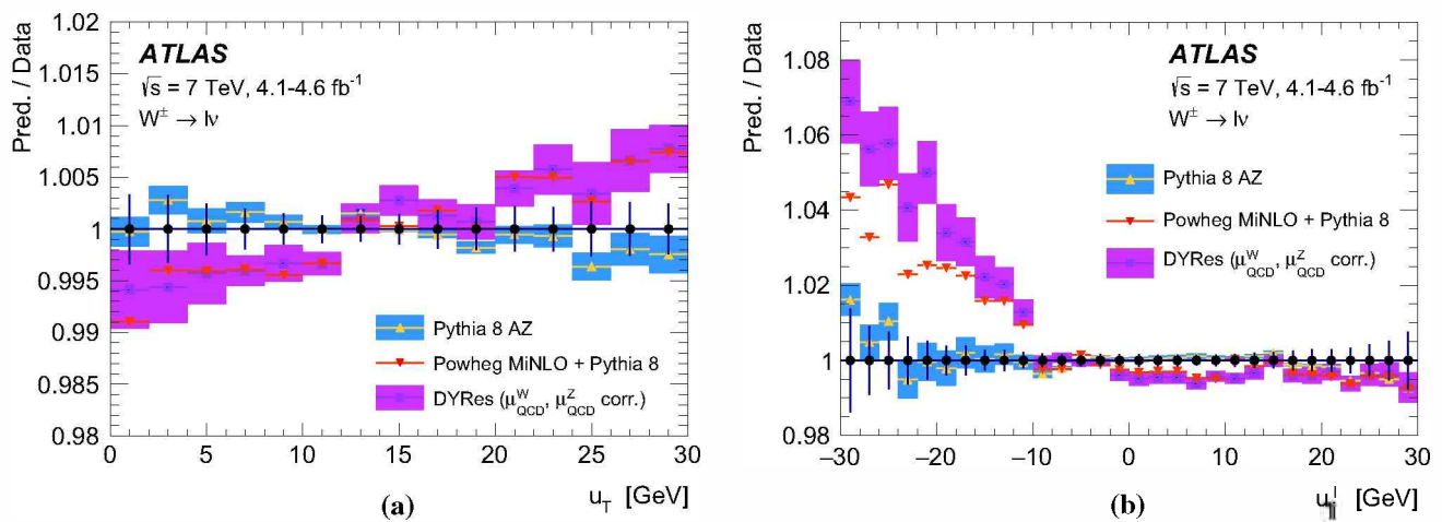
Fig. 22 Ratio between the predictions of PYTHIA 8 AZ, DYRes and POWHEG MINLO+PYTHIA 8 and the data for the a u_T and b u_1^{|} distributions in W \rightarrow \ell\nu events. The W -boson rapidity distribution is reweighted according to the NNLO prediction. The error bars on the data points display the total experimental uncertainty, and the band around
