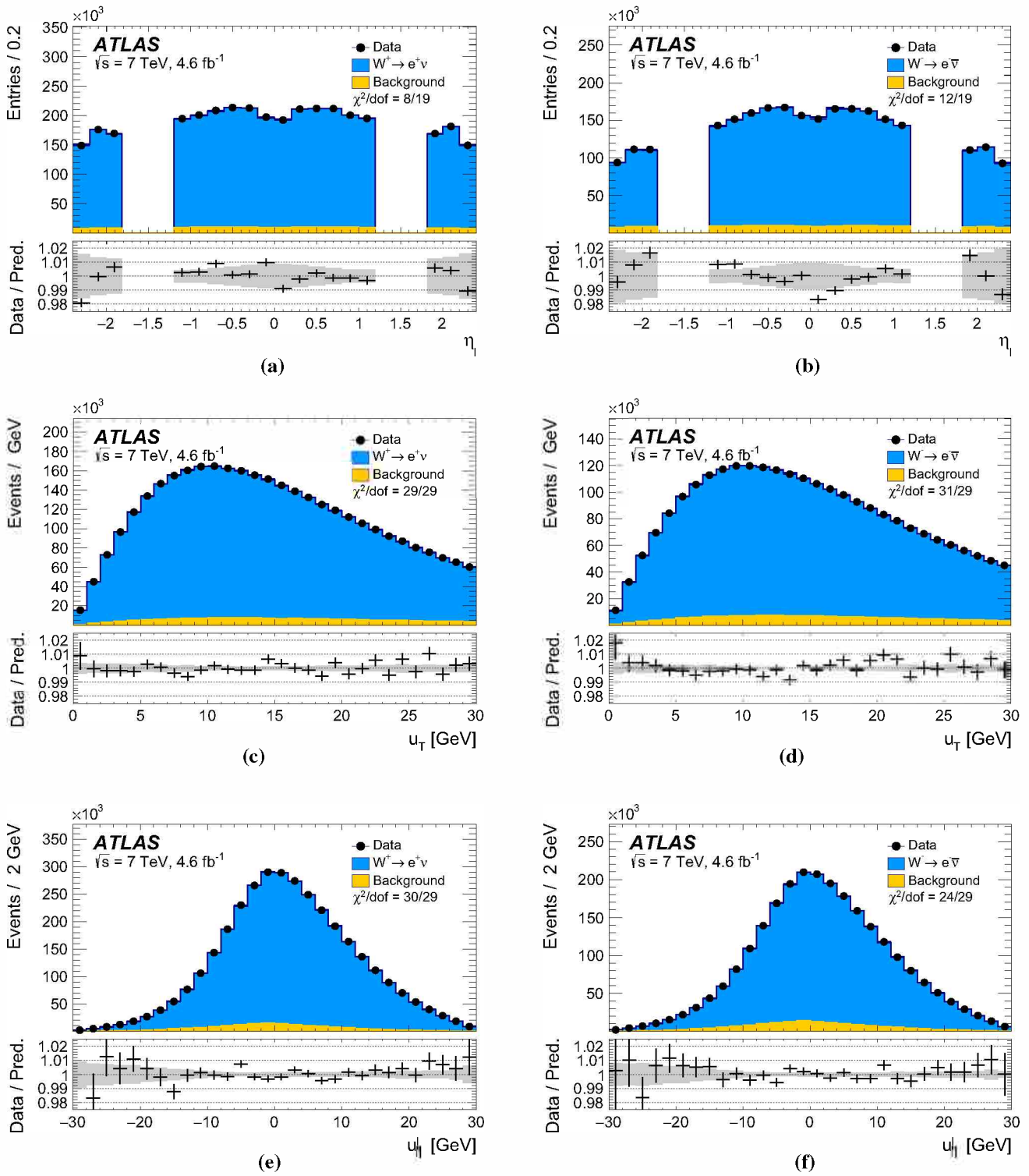
Fig. 19 The a, b \eta , (c,d) u_T , and e, f u_{\parallel} distributions for a, c, e W^+ events and b, d, f W^- events in the electron decay channel. The data are compared to the simulation including signal and background contributions. Detector calibration and physics-modelling corrections are applied to the simulated events. The lower panels show the data-to-
