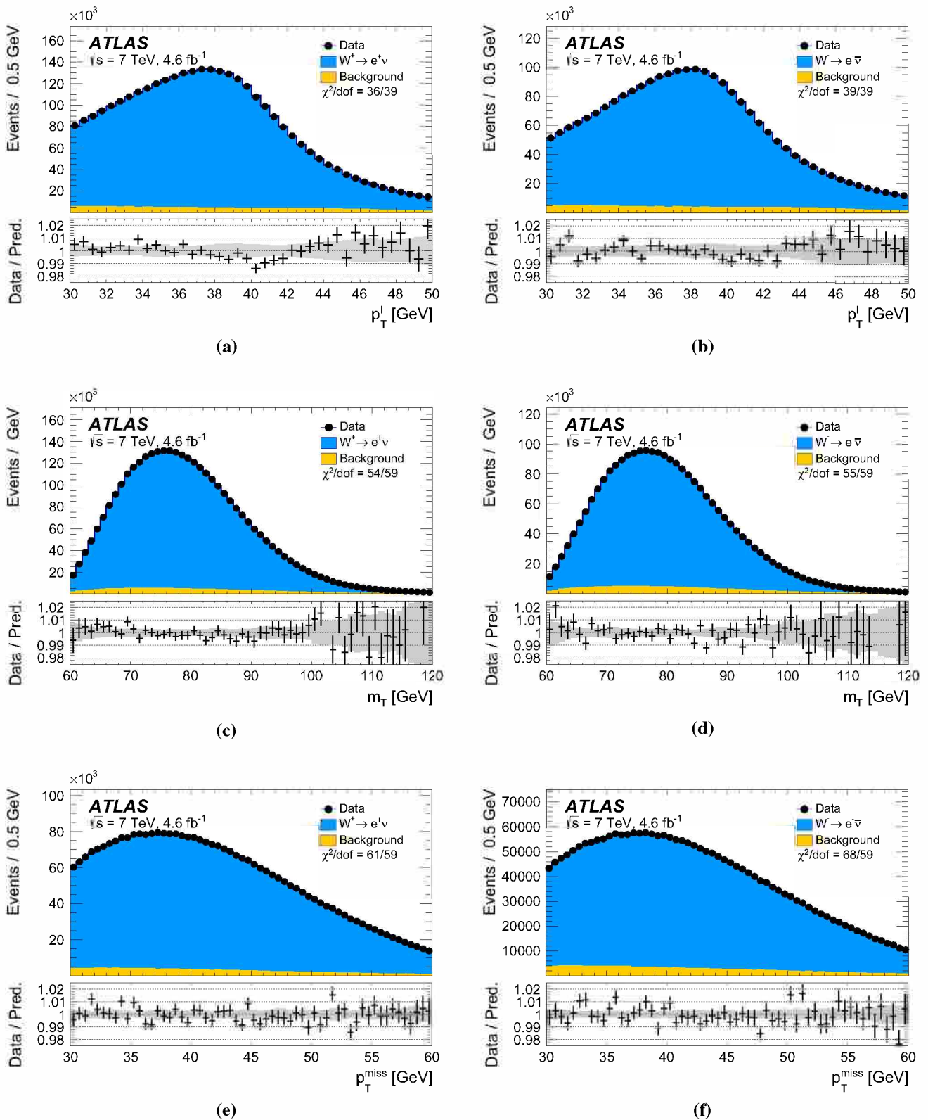
Fig. 24 The a , b p_T^e , c , d m_T , and e , f p_T^{\text{miss}} distributions for a , c , e W^+ events and b , d , f W^- events in the electron decay channel. The data are compared to the simulation including signal and background contributions. Detector calibration and physics-modelling corrections are applied to the simulated events. For all simulated distributions, m_W is set according to the overall measurement result. The lower panels
