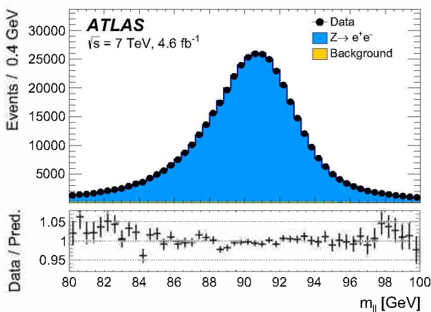
Fig. 9 Dielectron invariant mass distribution in Z \rightarrow ee events. The data are compared to the simulation including signal and backgrounds. Corrections for energy resolution, and for reconstruction, identification, isolation and trigger efficiencies are applied to the simulation; energy-scale corrections are applied to the data. Background events contribute less than 0.2% of the observed distribution. The lower panel shows the data-to-prediction ratio, with the error bars showing the statistical uncertainty
