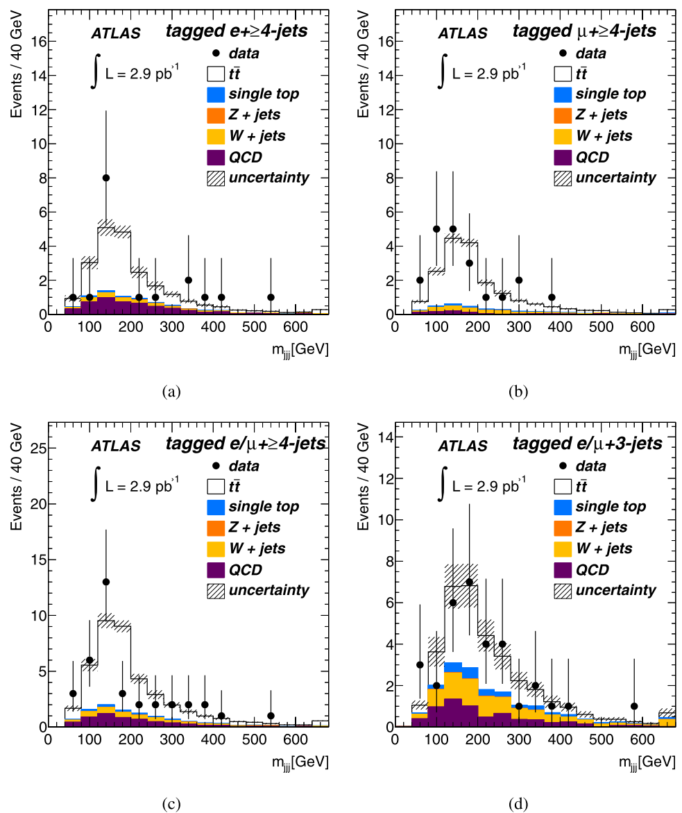
Fig. 3 Distributions of the invariant mass of the 3-jet combination having the highest p_T for a the \geq 4 -jet tagged e + \text{jets} sample, b the \geq 4 -jet tagged \mu + \text{jets} sample, c the \geq 4 -jet tagged samples combined and d the combined 3-jet tagged sample. The data is compared to the sum of all expected contributions. For the totals shown, simulation estimates are used for all contributions except QCD multi-jet, where a data-driven technique is used. The background uncertainty on the total expectation is represented by the hatched area
