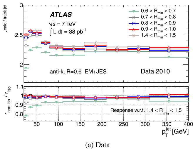
Fig. 75 Ratio of calorimeter jet p_T^{\text{jet}} to the matched track jet p_T as a function of calorimeter jet p_T^{\text{jet}} for anti- k_t jets with R = 0.6 in data (a) and Monte Carlo simulations (b) for different R_{\text{min}} values. The lower
