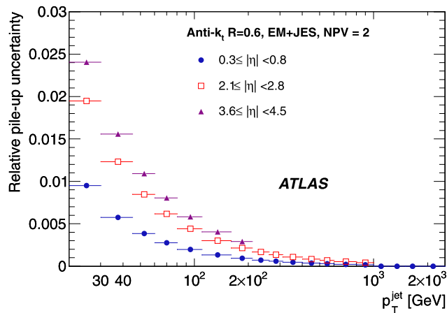
Fig. 20 Relative JES uncertainty from pile-up for anti- k_i jets with R = 0.6 in the case of two measured primary vertices, N_{\text{PV}} = 2 , for central ( 0.3 \leq |\eta| < 0.8 , full circles), endcap ( 2.1 \leq |\eta| < 2.8 , open squares) and forward ( 3.6 \leq |\eta| < 4.5 , full triangles) jets as a function of jet p_{\text{T}}^{\text{jet}}
