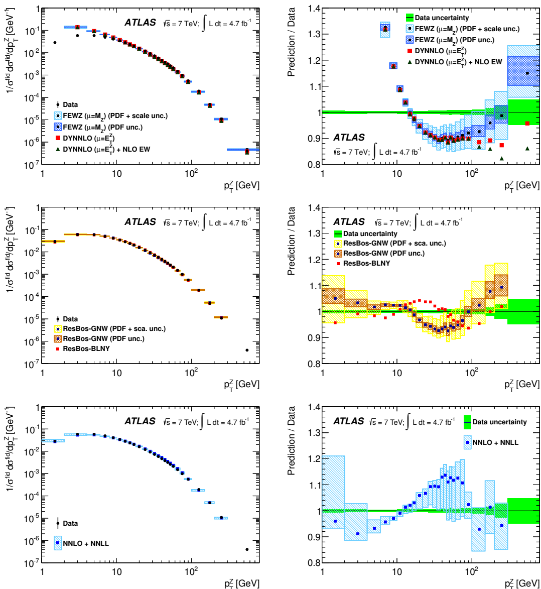
Figure 7. Left: comparison of the p_T^Z distributions predicted by different computations: FEWZ and DYNLO (top), RESBOS (middle) and the NNLO+NNLL calculation of ref. [21] (bottom) with the Born-level combined measurement, inclusively in y_Z . Right: ratios between these predictions and the combined measurement.
