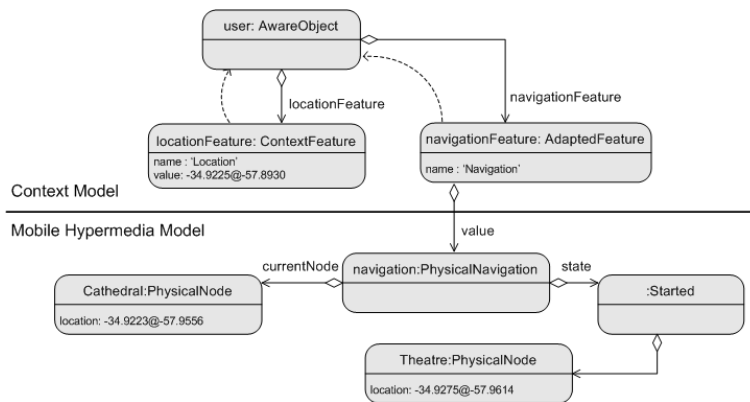
Figure 10 Context model for an extended mobile hypermedia application.
