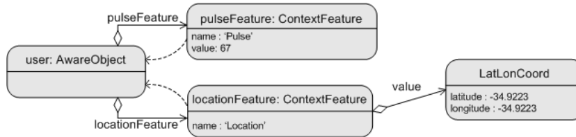
Figure 3 A simple context model.
