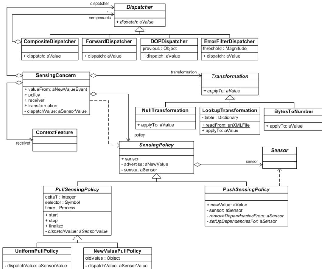
Figure 4 A class diagram of the sensing layer.
