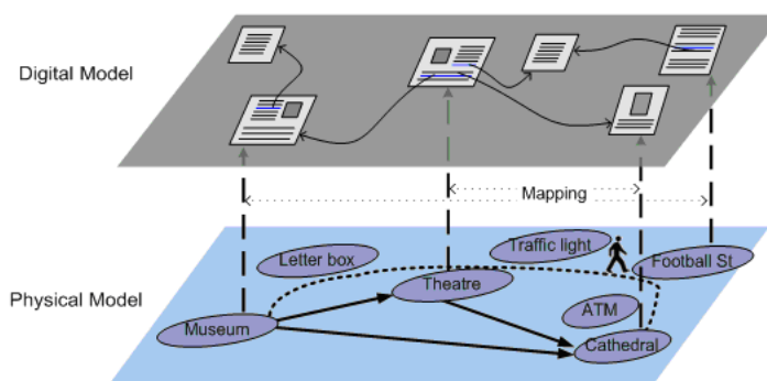
Figure 7 Nodes in a mobile hypermedia application.
