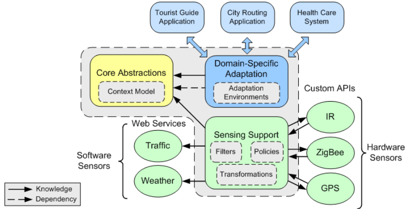
Figure 2 Overview of the Context-Aware architecture.
