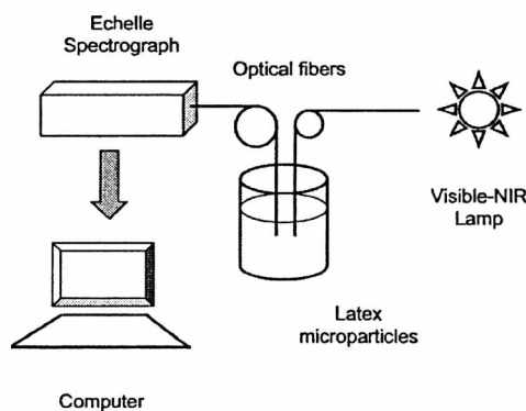
Fig. 2. Experimental setup.
