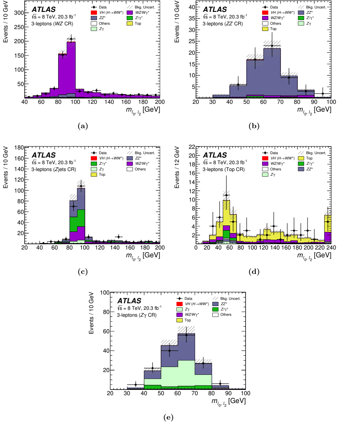
Figure 2. Distributions of the invariant mass of leptons l_0 and l_2 , defined in section 2, in the five CRs defined in the 3l channel: (a) 3l -WZ CR, (b) 3l -ZZ CR, (c) 3l -Zjets CR, (d) 3l -Top CR and (e) 3l - Z\gamma CR. Data (points) are compared to the background plus VH(H \rightarrow WW^*) ( m_H=125 GeV) signal expectation (stacked filled histograms), where the background contributions are normalised by applying the normalisation factors shown in table 7. The hatched area on the histogram represents total uncertainty, both statistical and systematic (see section 7), on the total background estimate. The last bin includes overflows.
