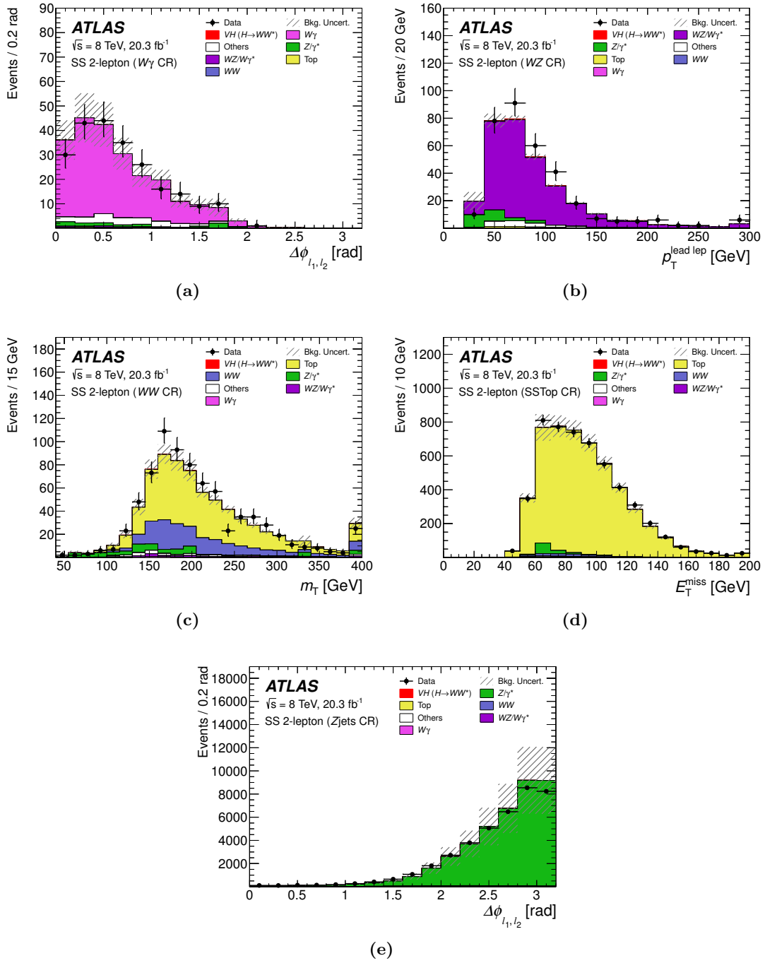
Figure 5. Distribution of relevant variables in the control regions in the 2\ell -SS channel: (a) azimuthal angle between the two leptons \Delta\phi_{\ell_1\ell_2} in the 2\ell - W\gamma CR, (b) transverse momentum of the leading lepton in the 2\ell - WZ CR, (c) transverse mass m_T in the 2\ell - WW CR, (d) missing transverse momentum E_T^{\text{miss}} in the 2\ell -SSTop CR and (e) \Delta\phi_{\ell_1\ell_2} , in the 2\ell -Zjets CR. Data (points) are compared to the background plus VH(H\rightarrow WW^*) ( m_H=125 GeV) signal expectation (stacked filled histograms), where the background contributions are normalised by applying the normalisation factors shown in table 7. The hatched area on the histogram represents total uncertainty, both statistical and systematic (see section 7), on the total background estimate. The last bin includes overflows.
