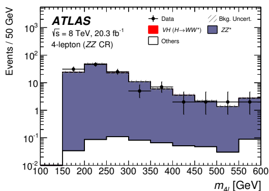
Figure 3. Distribution of the 4-lepton invariant mass m_{4\ell} in the 4\ell - ZZ CR control region. Data (points) are compared to the background plus VH(H \rightarrow WW^*) ( m_H=125 GeV) signal expectation (stacked filled histograms), where ZZ^* events are normalised by applying the normalisation factor shown in table 7. The hatched area on the histogram represents total uncertainty, both statistical and systematic (see section 7), on the total background estimate. The last bin includes overflows.
