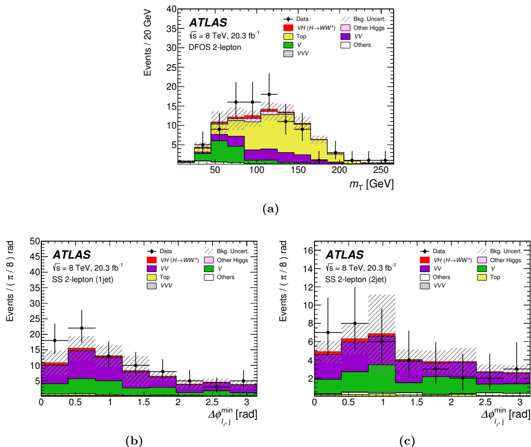
Figure 8. Distributions of relevant quantities for the 2\ell analyses using the 8 TeV data sample: (a) transverse mass m_T in the 2\ell -DFOS SR, the smallest azimuthal opening angle between a lepton and a jet, \phi_{\ell,j}^{\min} , (b) in the 2\ell -SS1jet and (c) 2\ell -SS2jet SRs. The distributions are shown with all the selections applied except for the one on the displayed variable. Data (points) are compared to the background plus the VH(H \rightarrow WW^*) ( m_H = 125 GeV) signal expectation (stacked filled histograms), where the background components are normalised by applying the normalisation factors shown in table 7. The hatched area on the histogram represents the total uncertainty on the background estimate including the statistical and systematic uncertainties added in quadrature.
