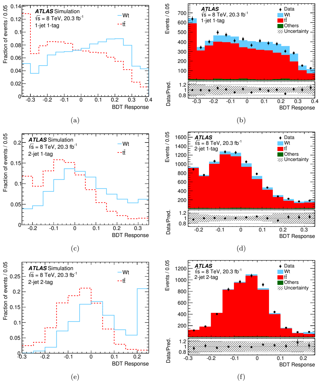
Figure 7. BDT response for (a, b) 1-jet 1-tag, (c, d) 2-jet 1-tag and (e, f) 2-jet 2-tag events. Each contribution is normalised to unit area in (a, c, e) and to its expectation in (b, d, f). The hatched area represents the sum in quadrature of the statistical and systematic uncertainties. The first bin includes the underflow and the last bin the overflow.
