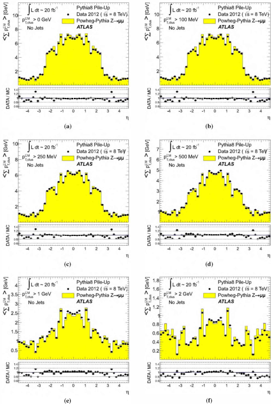
Fig. 23 The average \langle \sum p_{T,clus}^{EM} \rangle of clusters at the EM scale, calculated as function of \eta using Eq. (41), for clusters with a p_{T,clus}^{EM} > 0 , b p_{T,clus}^{EM} > 100 \text{ MeV} , c p_{T,clus}^{EM} > 250 \text{ MeV} , d p_{T,clus}^{EM} > 500 \text{ MeV} , e p_{T,clus}^{EM} > 1 \text{ GeV} , and f p_{T,clus}^{EM} > 2 \text{ GeV} . Results are obtained from a
