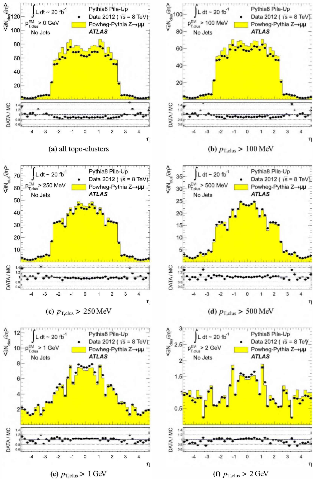
Fig. 25 Average topo-cluster number density \langle \partial N / \partial \eta \rangle as a function of \eta_{\text{clus}} , for clusters with p_{T,\text{clus}}^{\text{EM}} > p_{T,\text{min}} , for various p_{T,\text{min}} values. Results are obtained from a 2012 Z \rightarrow \mu\mu sample without jets with
