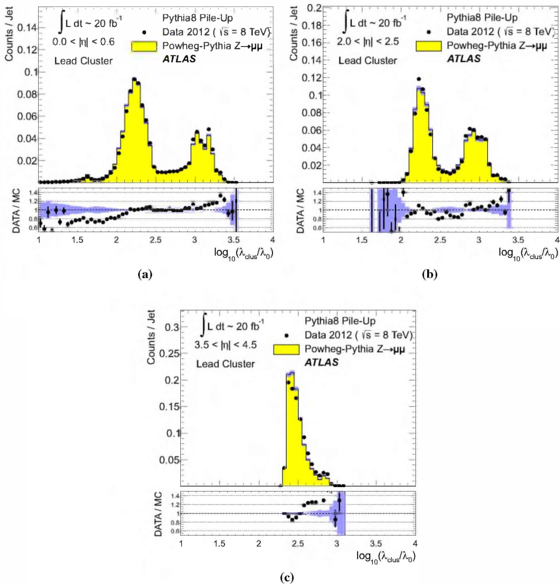
Fig. 36 The distribution of the leading topo-cluster depth location measure \log_{10}(\lambda_{clus}/\lambda_0) in fully calibrated jets reconstructed with the anti- k_t algorithm with R = 0.4 and 30\text{ GeV} < p_{T,jet}^{LCW+JES} < 40\text{ GeV} in regions of a the central ( |\eta_{jet}| < 0.6 ), b the end-cap ( 2.0 < |\eta_{jet}| < 2.5 ), and the c forward ( 3.5 < |\eta_{jet}| < 4.5 ) calorimeters in ATLAS. Data is compared to MC simulations with
