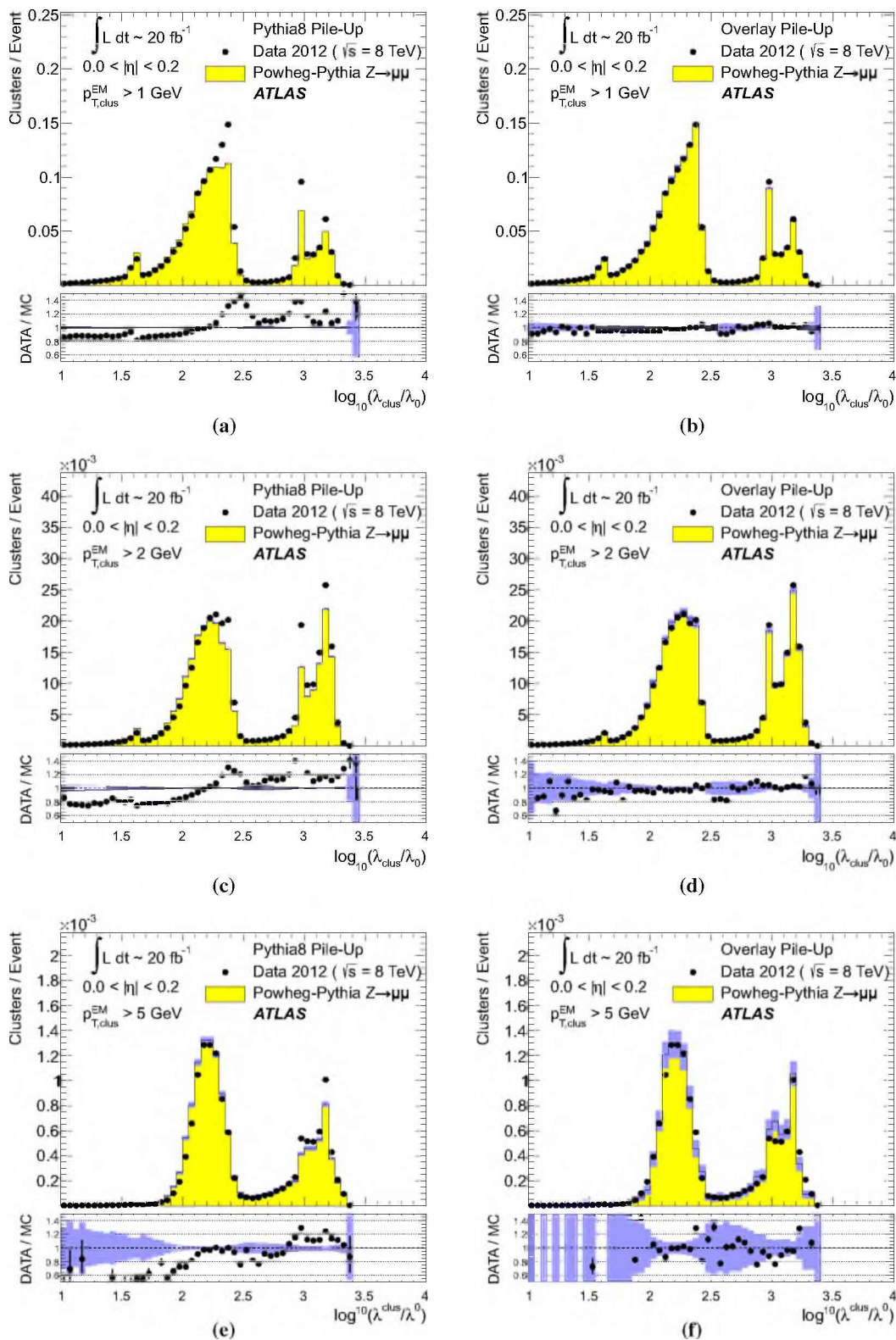
Fig. 29 The distribution of the topo-cluster depth location, measured in terms of \log_{10}(\lambda_{clus}/\lambda_0) , for selected topo-clusters within |\eta_{clus}| < 0.2 and with a transverse momentum p_{T,clus}^{EM} , evaluated on the EM scale, larger than various thresholds. Results are shown for an inclusive Z \rightarrow \mu\mu event sample recorded in 2012. Data are compared to distributions from MC simulations including fully simulated pile-up for
