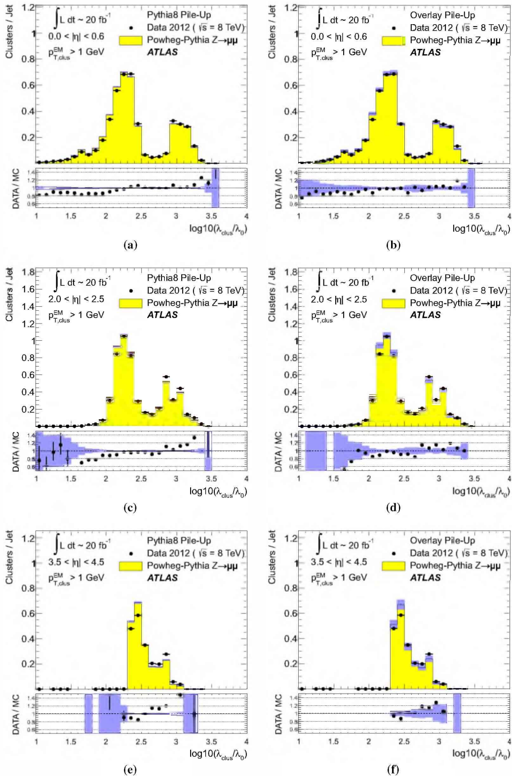
Fig. 35 The distribution of the depth location, measured in terms of \log_{10}(\lambda_{clus}/\lambda_0) with \lambda_0 = 1 mm, of topo-clusters with p_{T,clus}^{EM} > 1 GeV in jets reconstructed with the anti- k_r algorithm with R = 0.4 and with 30 \text{ GeV} < p_{T,jet}^{LCW+JES} < 40 \text{ GeV} in Z \rightarrow \mu\mu events in 2012 data and MC simulations with (a, c, e) fully simulated pile-up and with (b, d, f) overlaid pile-up from data. Distributions are shown for jets in the (a, b)
