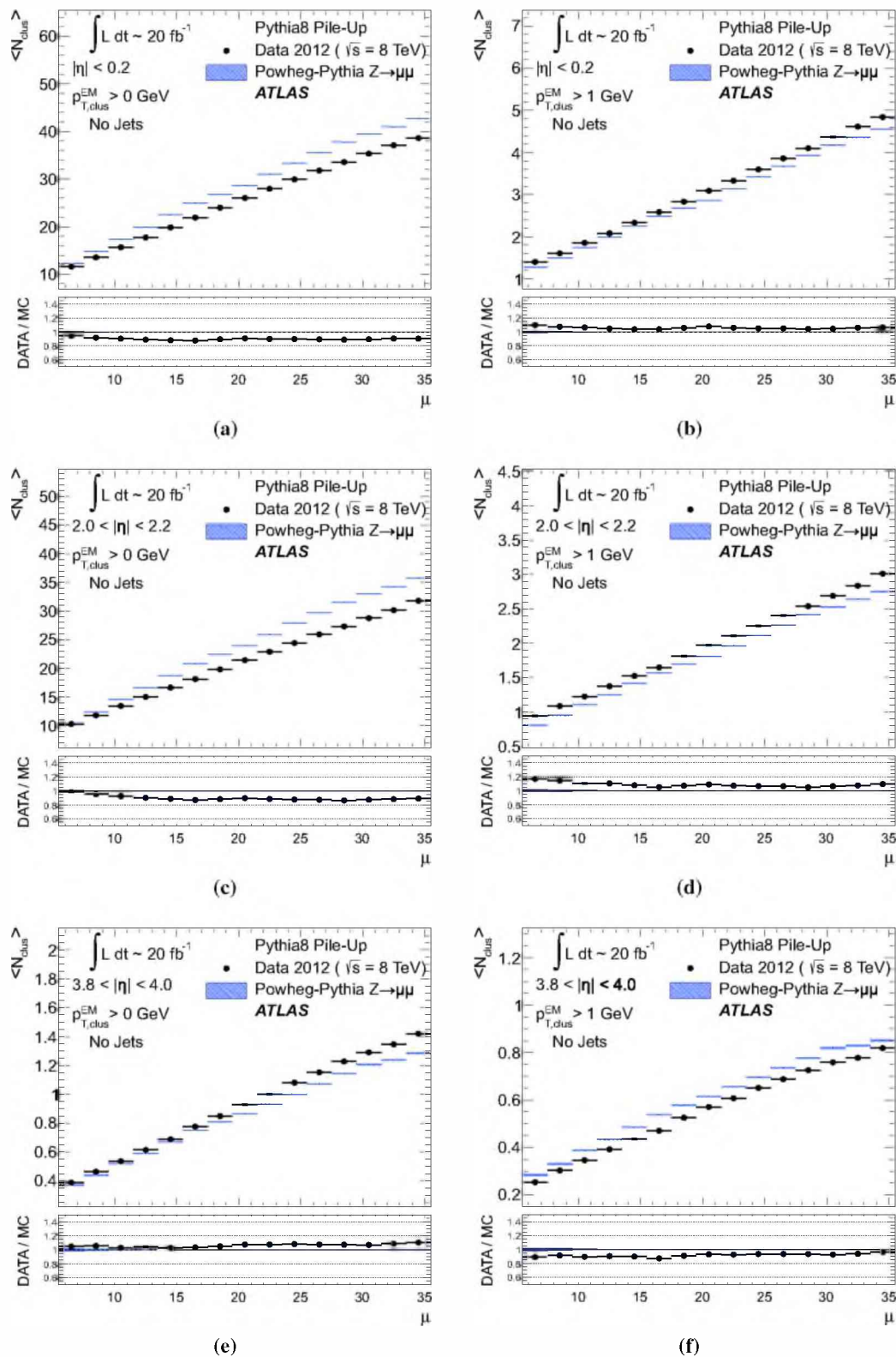
Fig. 27 The dependence of the average number of positive-energy topoclusters on the pile-up activity measured by the number of proton-proton collisions per bunch crossings \mu in several regions of the detector is shown in a, b for |\eta| < 0.2 , in c, d for 2.0 < |\eta| < 2.2 , and in e, f for 3.8 < |\eta| < 4.0 . Plots a, c and e show the results for counting all clusters with p_{T,\text{clus}}^{\text{EM}} > 0 , while b, c and f show the results for only
