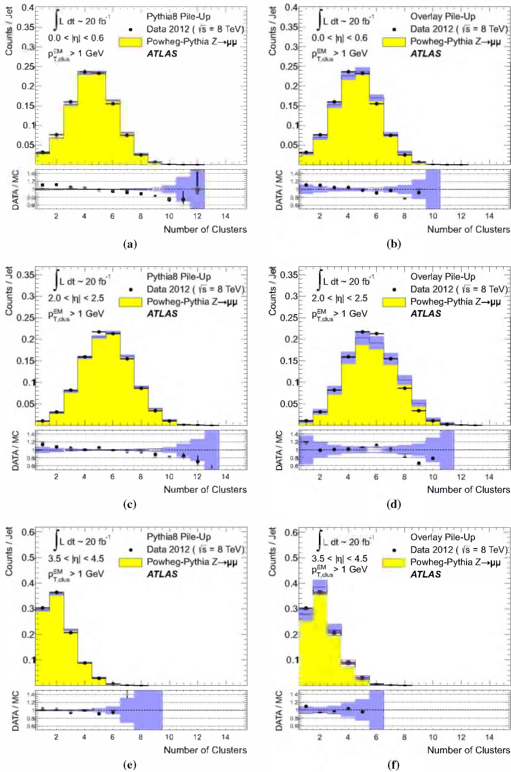
Fig. 32 The distribution of the number of topo-clusters with p_{T,clus}^{EM} > 1 \text{ GeV} inside anti- k_t jets with R = 0.4 in the (a, b) central ( |\eta| < 0.6 ), the (c, d) end-cap ( 2.0 < |\eta| < 2.5 ), and the (e, f) forward detector region ( 3.5 < |\eta| < 4.5 ) of ATLAS. Shown are results from the analysis of Z \rightarrow \mu\mu events with at least one jet with 30 \text{ GeV} < p_T < 40 \text{ GeV} in 2012 data and MC simulations with fully simulated pile-up in a, c
