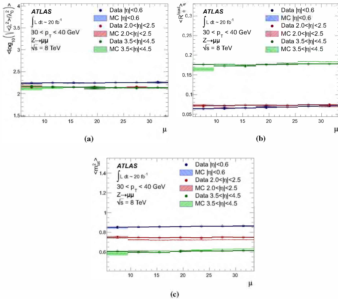
Fig. 44 The average pile-up dependence of various geometric observables reconstructed from the leading topo-cluster in anti- k_t jets reconstructed with R = 0.4 and 30 \text{ GeV} < p_{T,\text{jet}}^{\text{LCW+JES}} < 40 \text{ GeV} in Z \rightarrow \mu\mu events in 2012 data and MC simulations with fully simulated pile-up. The average cluster length, represented by \log_{10}(\langle \lambda^2 \rangle / \lambda_0^2)^{1/2} with the reference scale \lambda_0 = 1 \text{ mm} , is shown as a function of \mu in a , for three detector regions. The average size \langle R_{\eta\phi}^{\text{lead}} \rangle of the lead-
