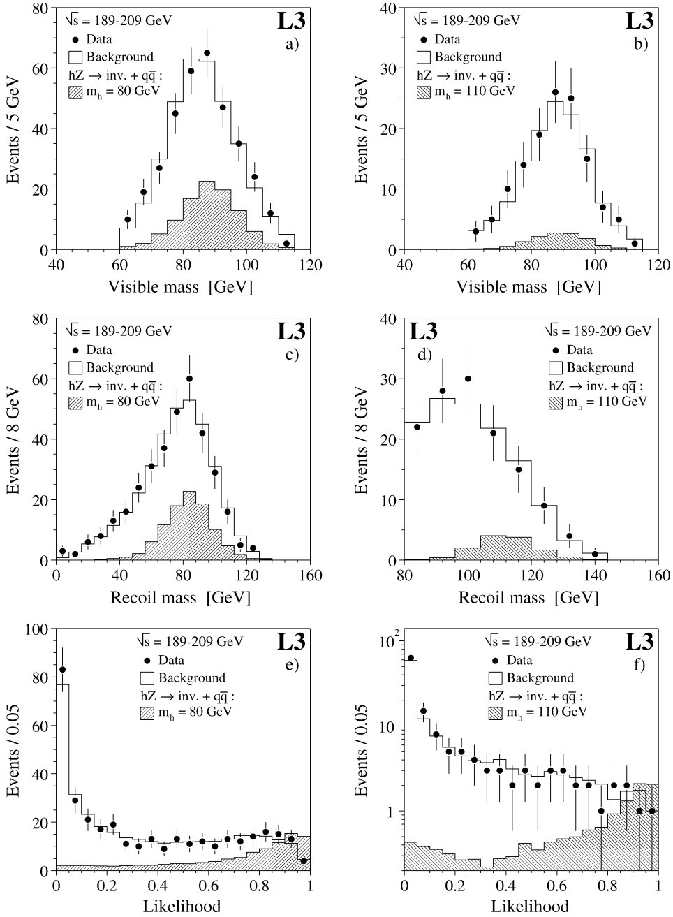
Fig. 2. Distributions of the visible and recoil masses for events selected by the light- and heavy-Higgs analyses of events with hadrons and missing energy. The dots represent the data, the open area the sum of all background contributions and the hatched histogram the expectation for a signal. The distributions of the final discriminants used in the analysis are also shown.
