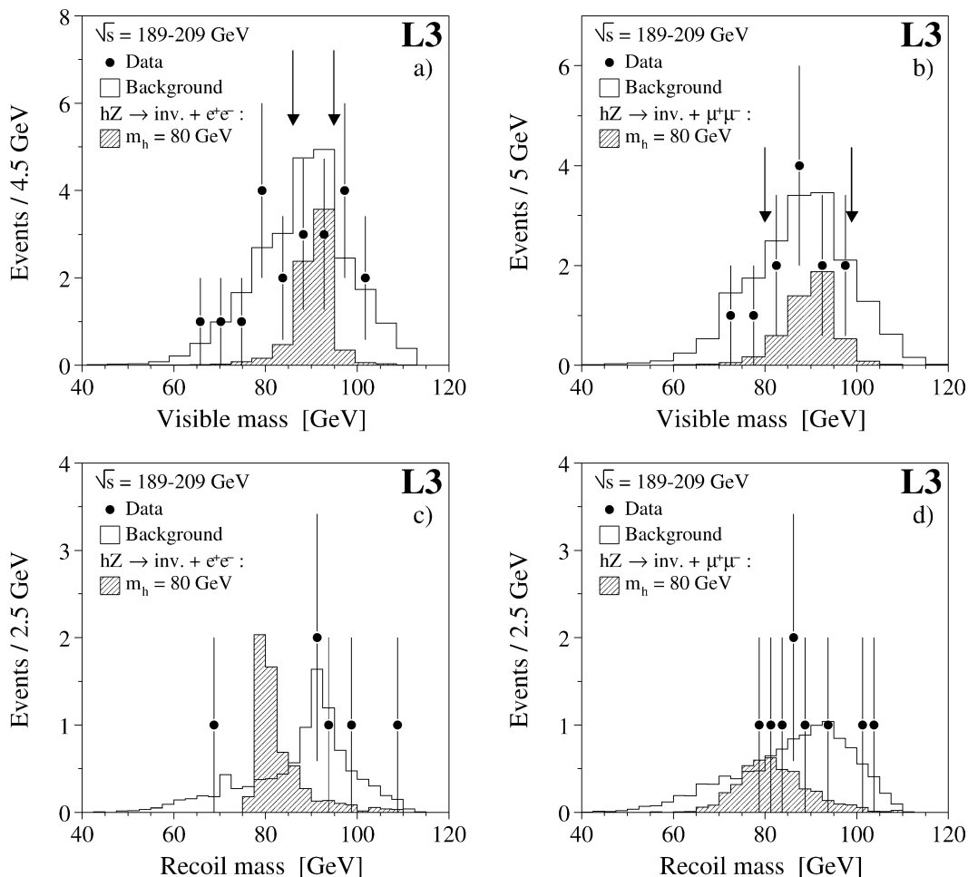
Fig. 4. Distributions of the visible mass of events selected by the analysis of final states with (a) electrons and missing energy and (b) muons and missing energy after. The selection criteria on the visible masses are illustrated by the arrows. Distributions of the recoil mass after the application of all cuts are shown in (c) for electrons and (d) for muons. The dots represent the data, the open area the sum of all background contributions and the hatched histogram the expectation for a signal.
