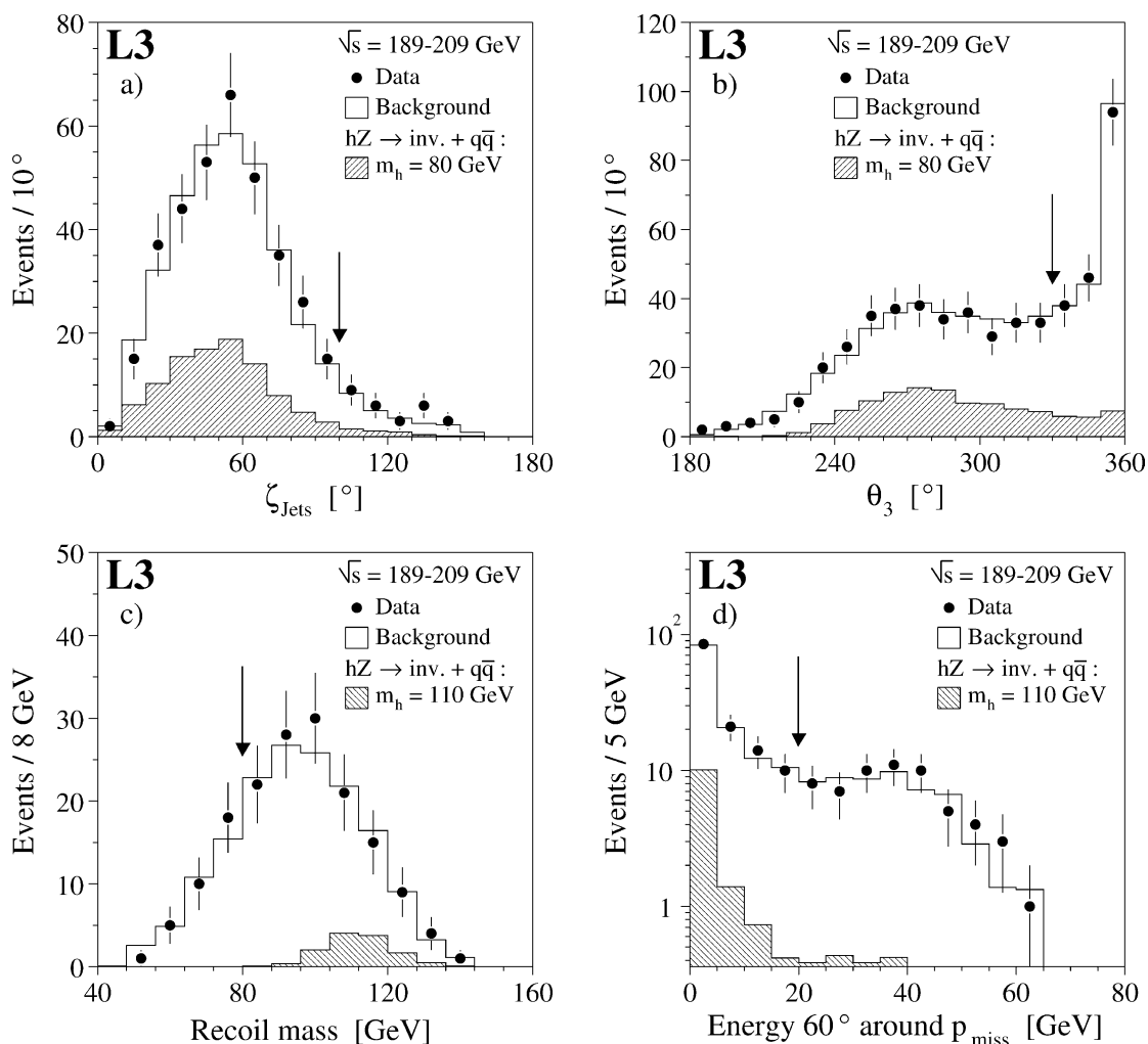
Fig. 1. Distributions of variables used in the selection of events with hadrons and missing energy. The dots represent the data, the open area the sum of all background contributions and the hatched histogram the expectation for a signal. The arrows represent the position of the selection criteria.
