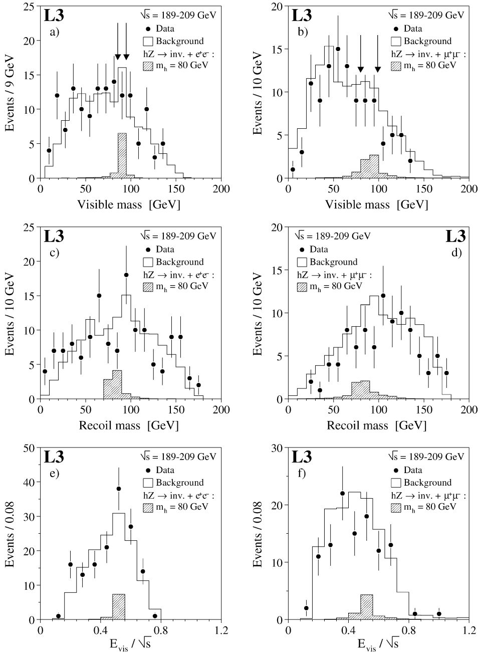
Fig. 3. Distributions of the visible and recoil masses and of the visible energy for events with electrons or muons and missing energy. The dots represent the data, the open area the sum of all background contributions and the hatched histogram the expectation for a signal. The selection criteria on the visible masses are illustrated by the arrows.
