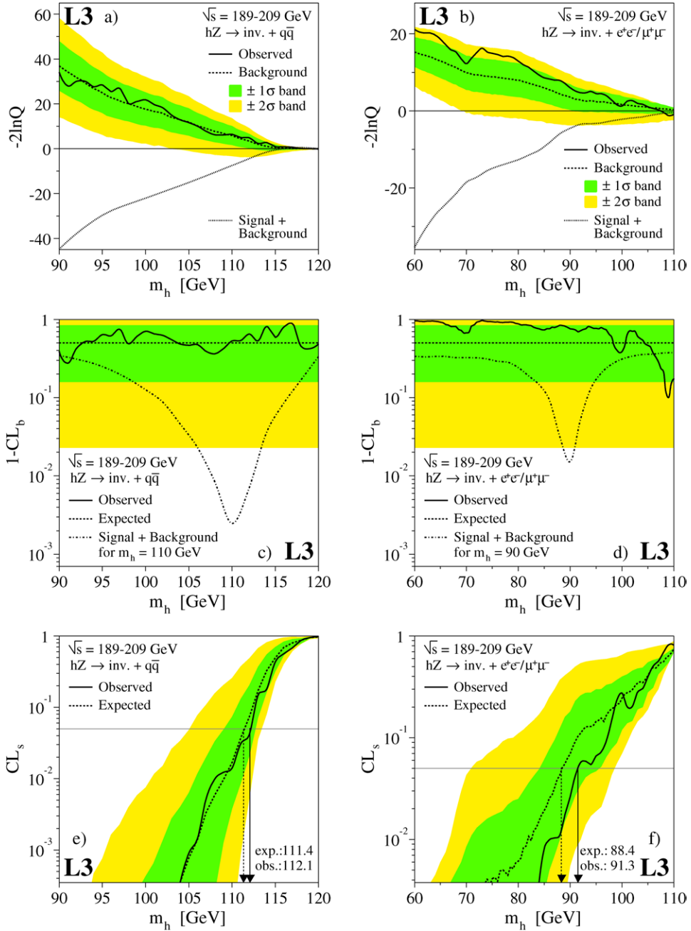
Fig. 5. Distributions as a function of m_h of the log-likelihood ratio for (a) the hadron and (b) the lepton analyses; of the 1 - CL_b estimator for (c) the hadron and (d) the lepton analyses; of the CL_s estimator for (e) the hadron and (f) the lepton analyses, together with the expected and observed lower limits on m_h .
