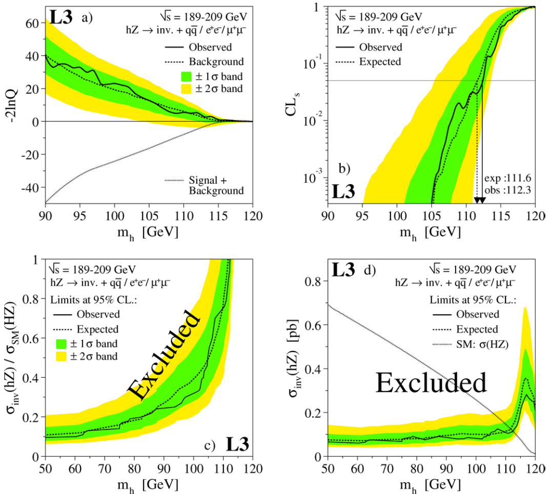
Fig. 6. Distributions as a function of m_h for the combination of the hadron and lepton analyses of (a) the log-likelihood; (b) the CL_s estimator with the expected and observed lower limits on m_h ; (c) upper limits on the ratio of the invisibly-decaying Higgs-boson cross section to the Standard Model one; (d) upper limits on the cross section for the production of an invisibly-decaying Higgs boson.
