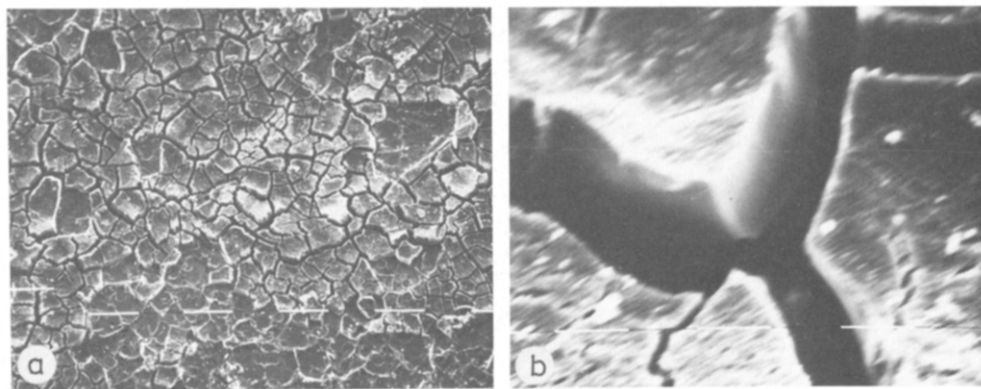
Fig. 2. Scanning electron micrographs of hydrated platinum oxide obtained after the SWPS treatment ( E_u = 2.4 V , E_1 = 0 V , \tau = 560 \mu s , t = 3 \text{ min} , 0.5 M H_2SO_4 , 30^\circ C ) Magnification (a) 100\times , (b) 1600\times
