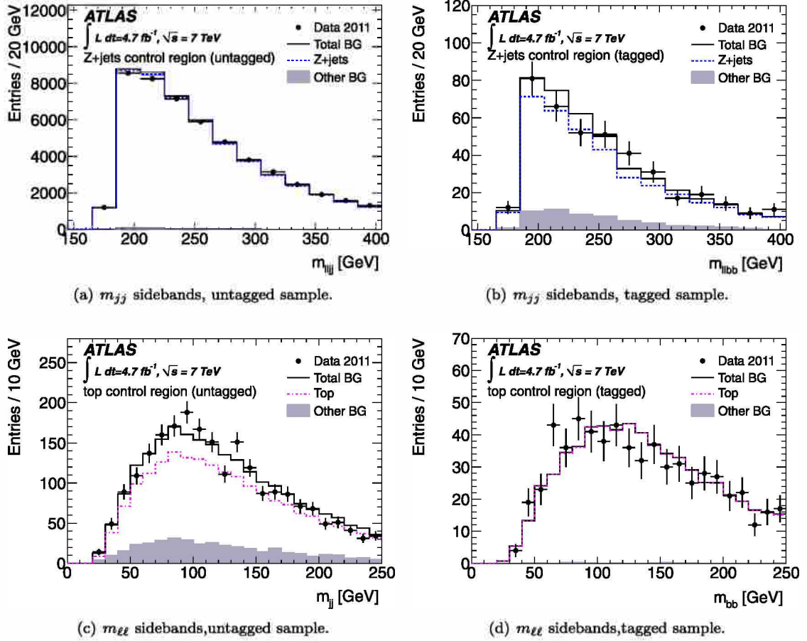
Fig. 2. Distributions from the background control samples, after application of scale factors, for the low- m_H selection. Top row: the \ell\ell jj invariant mass for 40 \text{ GeV} < m_{jj} < 70 \text{ GeV} or 105 \text{ GeV} < m_{jj} < 150 \text{ GeV} for (a) the untagged and (b) the tagged sample. Bottom row: the invariant mass of the jj system for events with 60 \text{ GeV} < m_{\ell\ell} < 76 \text{ GeV} or 106 \text{ GeV} < m_{\ell\ell} < 150 \text{ GeV} and E_T^{\text{mis}} > 50 \text{ GeV} for (c) the untagged sample and (d) the tagged sample.
