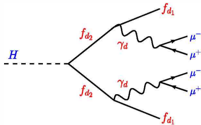
Fig. 1. Schematic picture of the Higgs boson decay chain, H \rightarrow 2(f_{d2} \rightarrow f_{d1}\gamma_d) . The Higgs boson decays to two hidden fermions ( f_{d2} ). Each hidden fermion decays to a \gamma_d and to a stable hidden fermion ( f_{d1} ), resulting in two muon jets from the \gamma_d decays in the final state.
