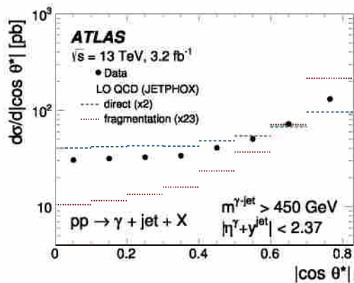
Fig. 4. Measured cross section for isolated-photon plus jet production (dots) as a function of |\cos\theta^*| ; the observable is constructed using the leading photon and the leading jet. For comparison, the LO QCD predictions from JETPHOX, normalised to the integrated measured cross section by the factors shown in parentheses, of direct (dashed lines) and fragmentation (dotted lines) processes are shown separately. The error bars are smaller than the marker size and, thus, not visible.
