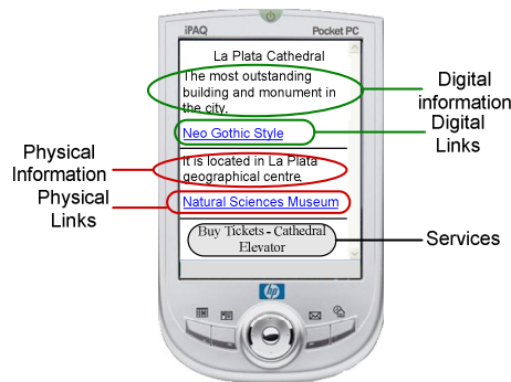
Figure 5. Interface of a PH application using a web browser.
