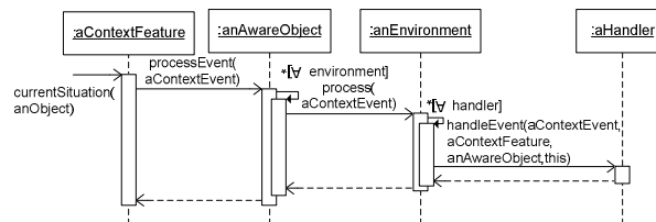
Figure 8. An interaction diagram showing the event propagation.
