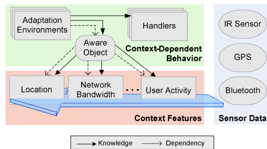
Figure 6. An architecture for handling context-dependent behavior.
