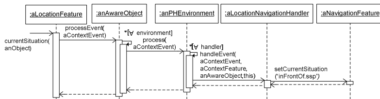
Figure 10. An interaction diagram showing a location change.
