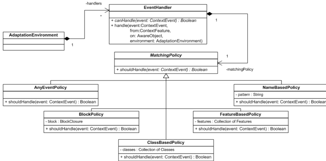
Figure 15. The MatchingPolicy hierarchy.
