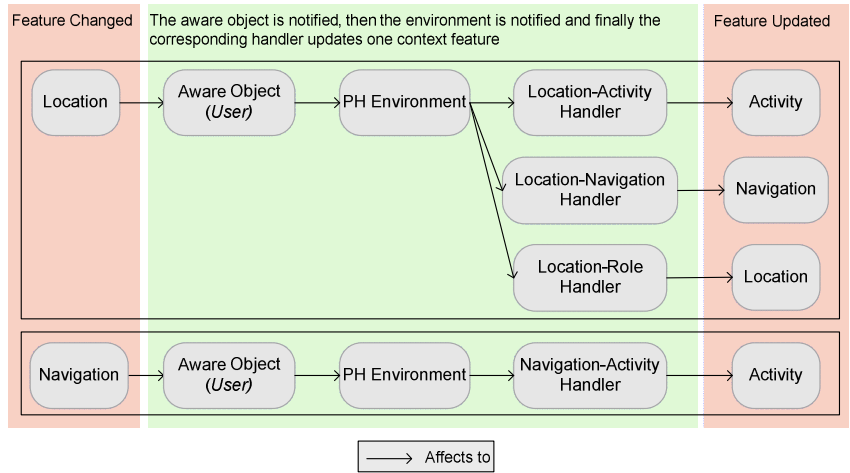
Figure 13. A complete diagram with the relations when contexts feature changes.
