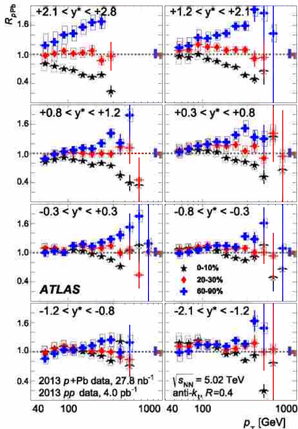
Fig. 5. Measured R_{pPb} values for R = 0.4 jets in p + \text{Pb} collisions in central (stars), mid-central (diamonds) and peripheral (crosses) events. Each panel shows the jet R_{pPb} in a different rapidity range. Vertical error bars represent the statistical uncertainty while the boxes represent the systematic uncertainties on the jet yields. The shaded boxes at the right edge of the R_{pPb} = 1 horizontal line indicate the systematic uncertainties on T_{pA} and the pp luminosity added in quadrature for (from left to right) peripheral, mid-central and central events.
