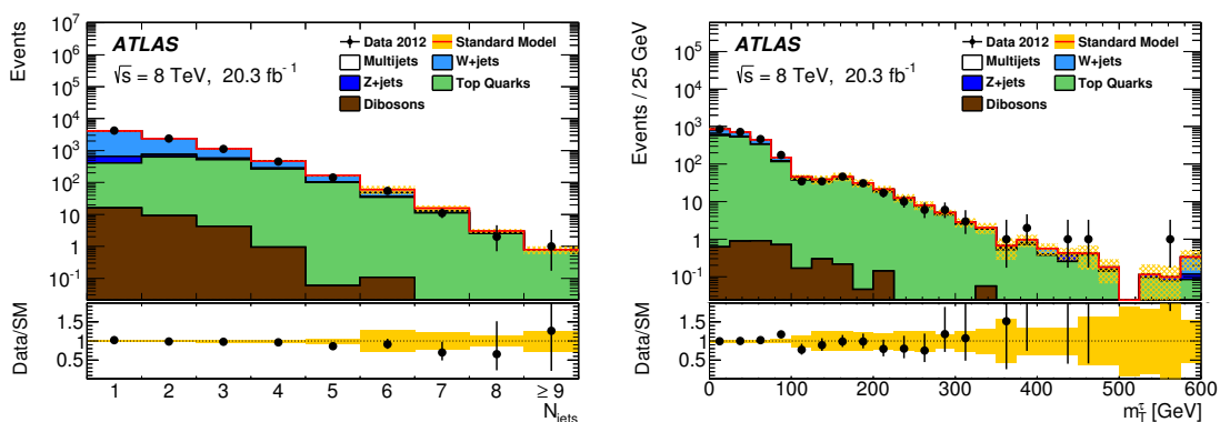
(a) N_{\text{jets}} distribution in inclusive W/Z and t\bar{t} region. (b) m_{\text{T}}^{\tau} distribution in the t\bar{t} validation region.
