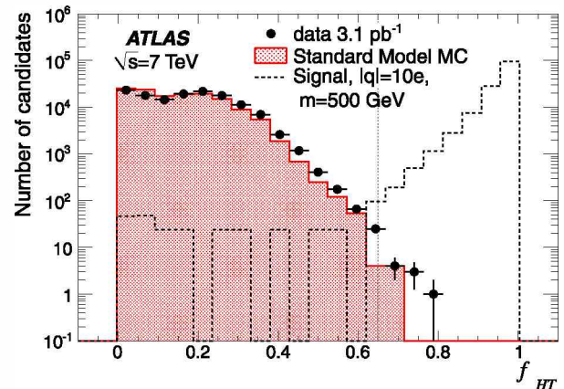
Fig. 2. Distribution of the fraction of TRT high-threshold hits for candidates satisfying the loose selection. Data (dots) are compared with area-normalised signal ( |q| = 10e and m = 500 \text{ GeV} , dashed line) and Standard Model background (shaded area) simulations. The dotted line shows the selection cut value.
