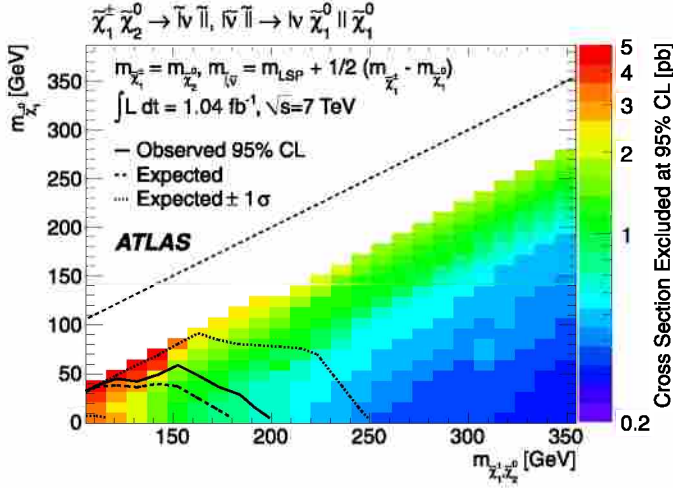
Fig. 2. 95% CL cross section upper limits (CL s ) in pb and observed and expected limit contours for \tilde{\chi}_1^\pm \tilde{\chi}_2^0 production in direct gaugino simplified models.
