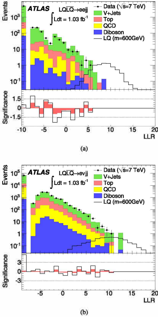
Fig. 3. LLR distributions for the eejj (a) and for the evjj (b) final states. The data are indicated with the points and the filled histograms show the SM background. The MJ background is estimated from data, while the other background contributions are obtained from simulated samples as described in the text. The LQ signal corresponding to a LQ mass of 600 GeV is indicated by a solid line, and is normalized assuming \beta = 1.0 (0.5) in the eejj ( evjj ) channel. The lowest bin corresponds to background events regions of the phase space for which no signal events are expected. The solid line (band) in the lower plots shows the Gaussian statistical (statistical + systematic) significance of the difference between data and the prediction.
