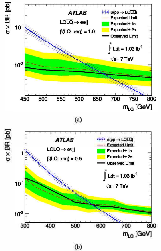
Fig. 4. 95% CL upper limit on the pair production cross section times branching ratio of the first generation leptoquarks for the eejj channel at \beta = 1.0 (a) and for the evjj channel at \beta = 0.5 (b). The solid lines indicate the individual observed limits, while the expected limits are indicated by the dashed lines. The theory prediction is indicated by the dotted line, which includes the systematic uncertainties due to the choice of the PDF and due to the renormalization and factorization scales. The dark green (light yellow) solid band contains 68% (95%) of possible outcomes from pseudo-experiments in which the yield is Poisson-fluctuated around the background-only expectation. (For interpretation of the references to color in this figure legend, the reader is referred to the web version of this Letter.)
