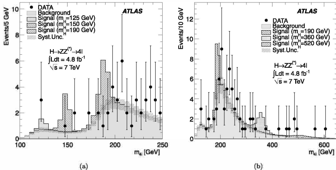
Fig. 4. m_{Al} distribution of the selected candidates, compared to the background expectation for (a) the 100–250 GeV mass range and (b) the full mass range of the analysis. Error bars represent 68.3% central confidence intervals. The signal expectation for several m_H hypotheses is also shown. The resolution of the reconstructed Higgs mass is dominated by detector resolution at low m_H values and by the Higgs boson width at high m_H .
