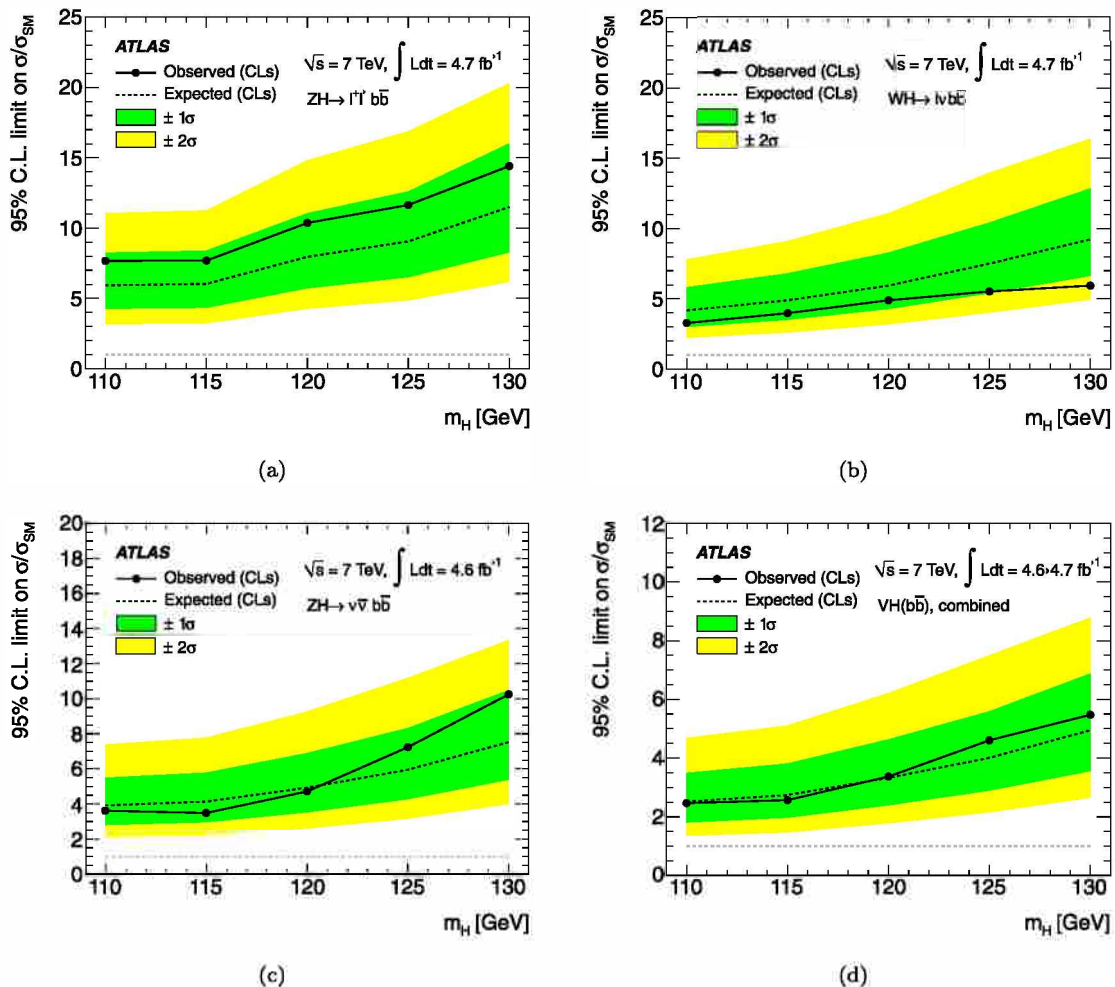
Fig. 5. Expected (dashed) and observed (solid line) exclusion limits for (a) the ZH \rightarrow \ell^+ \ell^- b\bar{b} , (b) WH \rightarrow \ell \nu b\bar{b} and (c) ZH \rightarrow \nu \bar{\nu} b\bar{b} channels expressed as the ratio to the SM Higgs boson cross section, using the profile-likelihood method with CL_s . The dark (green in the web version) and light (yellow in the web version) areas represent the \pm 1\sigma and \pm 2\sigma ranges of the expectation in the absence of a signal. (d) shows the 95% CL exclusion limits obtained from the combination of the three channels.
