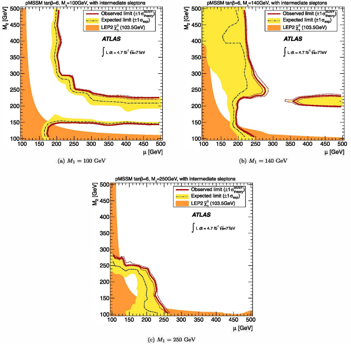
Fig. 3. 95% CL s exclusion limits in the \mu – M_2 mass plane of the pMSSM for (a) M_1 = 100 \text{ GeV} , (b) M_1 = 140 \text{ GeV} and (c) M_1 = 250 \text{ GeV} . The dashed and solid lines show the 95% CL s expected and observed limits, respectively, including all uncertainties except for the theoretical signal cross-section uncertainty (PDF and scale). The solid band around the expected limit shows the \pm 1\sigma result where all uncertainties, except those on the signal cross-sections, are considered. The \pm 1\sigma lines around the observed limit represent the results obtained when moving the nominal signal cross-section up or down by the \pm 1\sigma theoretical uncertainty.
