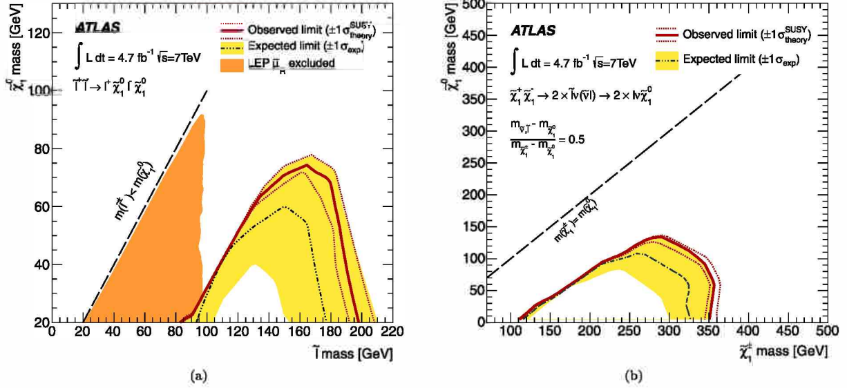
Fig. 2. 95% CL exclusion limits for \tilde{\ell}^\pm pair production in the m_{\tilde{\ell}} - m_{\tilde{\chi}_1^0} mass plane of (a) the direct slepton pMSSM and (b) \tilde{\chi}_1^\pm \tilde{\chi}_1^\mp pair production in the simplified model. The dashed and solid lines show the 95% CL exp and observed limits, respectively, including all uncertainties except for the theoretical signal cross-section uncertainty (PDF and scale). The solid band around the expected limit shows the \pm 1\sigma result where all uncertainties, except those on the signal cross-sections, are considered. The \pm 1\sigma lines around the observed limit represent the results obtained when moving the nominal signal cross-section up or down by the \pm 1\sigma theoretical uncertainty. Illustrated also in (a) is the LEP limit [28] on the mass of the right-handed smuon, \tilde{\mu}_R . The LEP limit is a conservative limit on slepton pair production: if right-handed slepton masses are excluded, left-handed sleptons of equivalent masses are automatically excluded. (For interpretation of the references to colour, the reader is referred to the web version of this Letter.)
