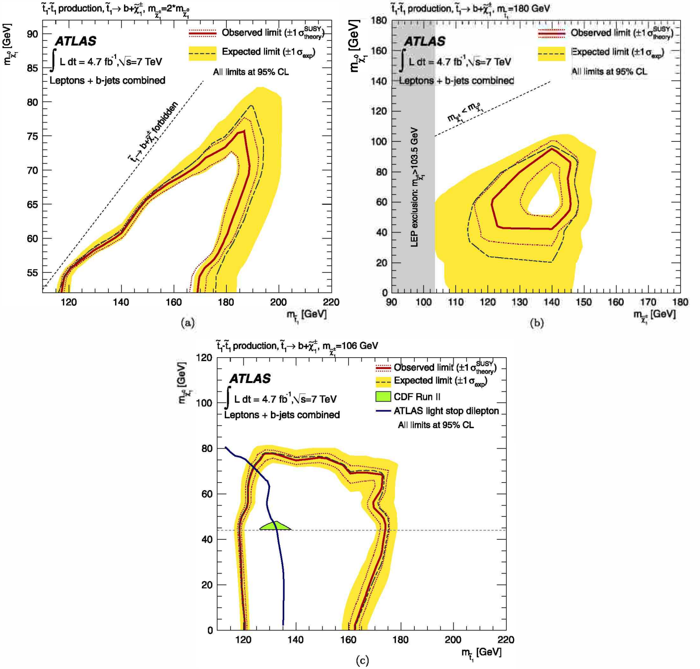
Fig. 2. Exclusion limits at 95% CL for the scenarios described in the text. The dashed (solid) lines show the expected (observed) limits, including all uncertainties except for the theoretical signal cross section uncertainty (PDF and scale). The bands around the expected limits show the \pm 1\sigma results. The lines around the observed limits represent the results obtained when moving the nominal signal cross section up or down by the \pm 1\sigma theoretical uncertainty. In (c), results are compared to previous limits from the Tevatron [16], where the lowest neutralino mass considered was 44 GeV (dotted line), and from ATLAS [17].
