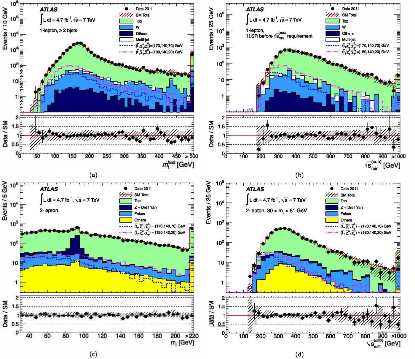
Fig. 1. The 1-lepton channel m_t^{\text{had}} distribution after all requirements except those on m_t^{\text{had}} and \sqrt{s_{\text{min}}^{(\text{sub})}} (a), and the \sqrt{s_{\text{min}}^{(\text{sub})}} distribution after all requirements except that on \sqrt{s_{\text{min}}^{(\text{sub})}} (b). For the 2-lepton channel, the m_{\ell\ell} distribution is shown after all requirements except those on m_{\ell\ell} and \sqrt{s_{\text{min}}^{(\text{sub})}} (c), and the \sqrt{s_{\text{min}}^{(\text{sub})}} distribution, before the requirements on \sqrt{s_{\text{min}}^{(\text{sub})}} itself (d). The last bin in each histogram contains the integral of all events with values greater than the upper axis bound. The hatched bands display the total uncertainties on the background expectation and the dashed lines show the expected distributions for two signal models. The bottom panels show the ratio of data to the expected background (points) and the total uncertainty on the background (hatched area).
