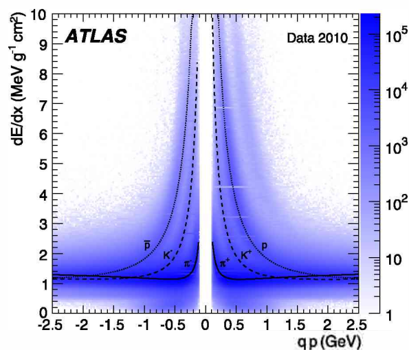
Fig. A.8. Greyscale-printing version of Fig. 1(left): Distribution of dE/dx versus charge times momentum for minimum bias collisions in a data sample from 2010. With tracks reconstructed for p_T > 100 MeV this sample is more suitable for the calibration of the Bethe-Bloch function than 2011 data in which tracks had a cut-off of p_T = 400 MeV. The distribution of the most probable value for pions (solid), kaons (dashed) and protons (dotted) are superimposed. The band due to deuterons is clearly visible.
