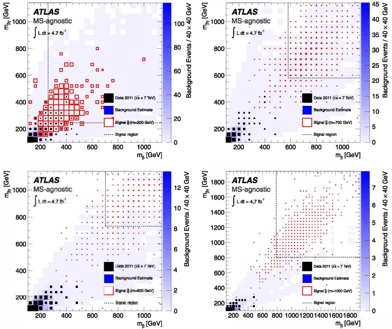
Fig. A.11. Examples of the m_{\beta\gamma} vs. m_\beta distributions for gluino R -hadrons with masses of 300, 700, 900 and 1000 GeV, with the MS-agnostic search. The figures show data, background and signal after \beta , \beta\gamma and p cuts. The dashed grey line highlights the counting window for each specific hypothesis, and is defined by requiring 90% of the signal to be within the window.
