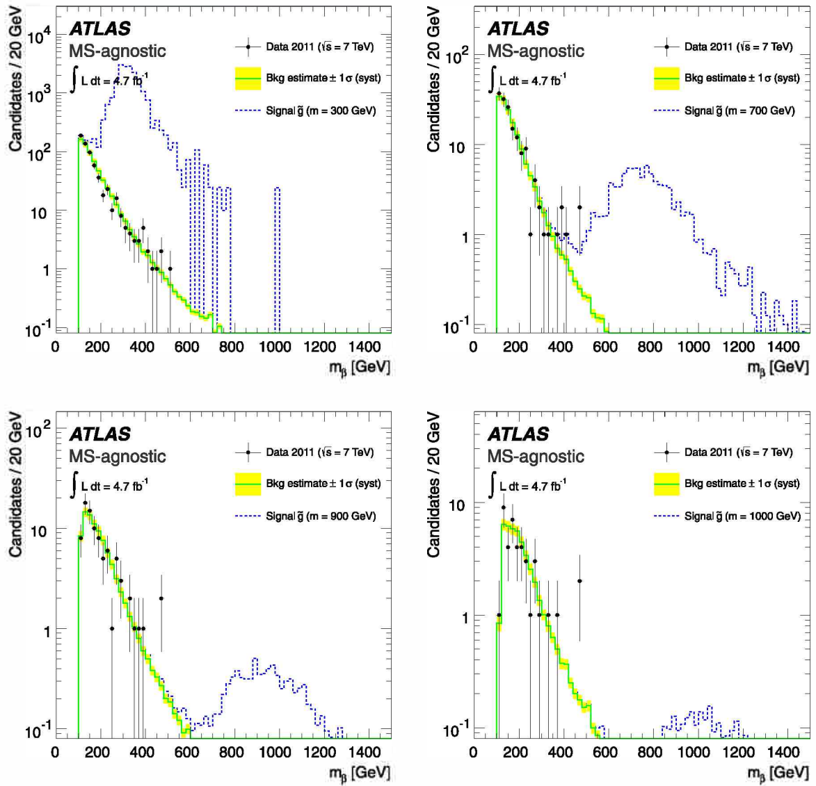
Fig. A.13. Observed data, background estimate and expected signal in the MS-agnostic R-hadron search, for various mass hypotheses (300, 700, 900 and 1000 GeV). The 1D histograms are projections of the 2D signal range with unconstrained m_{B\gamma} .
