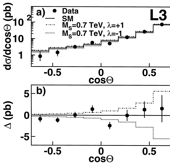
Fig. 4. a) Differential cross section for Bhabha scattering in data and the SM expectations. LSG modifications for M_S = 0.7 TeV are also displayed for \lambda = \pm 1 . b) Differences \Delta of the above with SM prediction.
