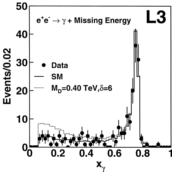
Fig. 1. Distribution of ratio of the photon energy to the beam energy for single photon events in data at \sqrt{s} = 183 GeV together with SM expectations. The effect of real graviton production with six extra space dimensions and M_D = 0.4 TeV is also shown.
