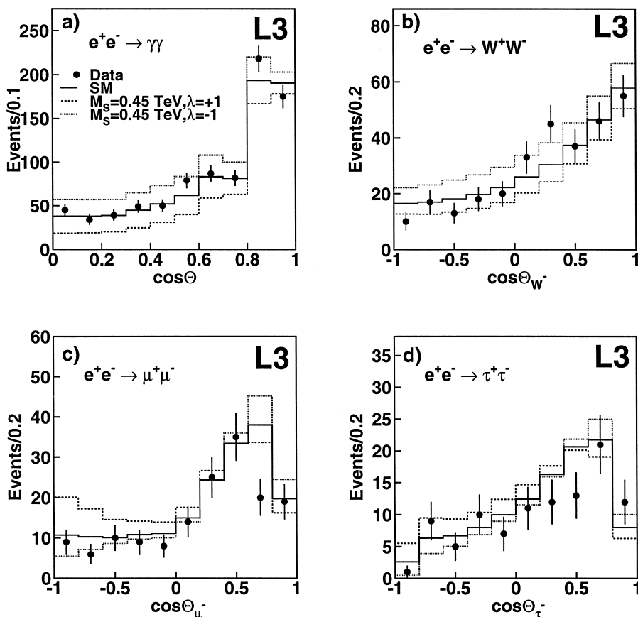
Fig. 2. Distributions of the polar angle for: (a) e^+e^- \rightarrow \gamma\gamma events selected at \sqrt{s} = 130\text{--}183 GeV, (b) semileptonic e^+e^- \rightarrow W^+W^- events, (c) e^+e^- \rightarrow \mu^+\mu^- and (d) e^+e^- \rightarrow \tau^+\tau^- processes. The last three plots refer to the \sqrt{s} = 183 GeV data sample only. Data, SM expectations and LSG effects for M_S = 0.45 TeV are shown.
