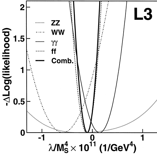
Fig. 3. Likelihood curves for \lambda/M_S^4 for all the processes described in the text and their combination.
