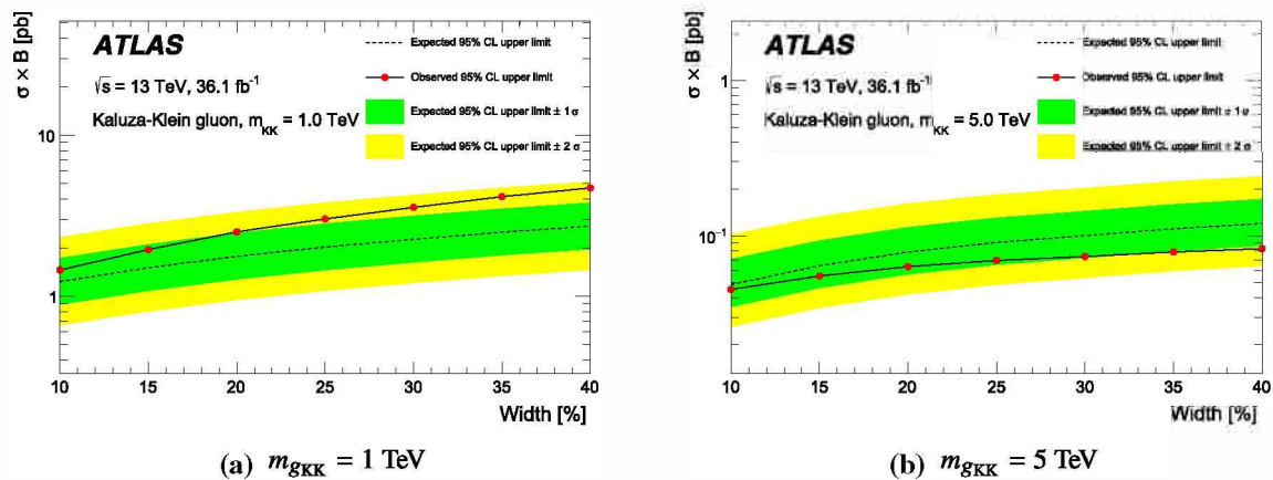
Fig. 18 The observed and expected cross-section 95% CL upper limits on the g_{KK} signal as a function of the resonance width for masses of a 1 TeV, and b 5 TeV
