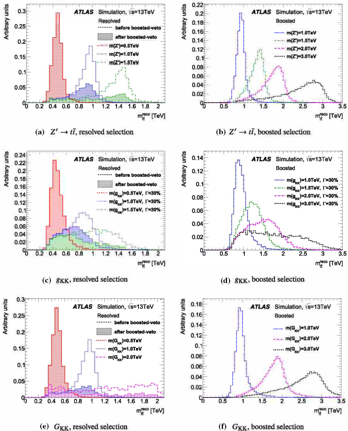
Fig. 3 Reconstructed top-quark pairs invariant mass, m_{tt}^{reco} , for simulated signal events satisfying the selection criteria. The Z' in the simulated samples used here has a width of 3% of its mass. The g_{KK} shown here has a width of 30% of its mass and the width of the G_{KK} width varies between 3 and 6% of its mass. The figure shows the distribution
