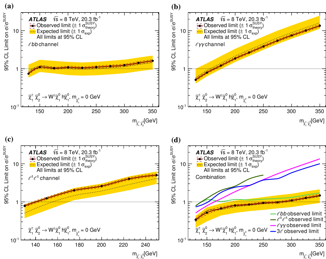
Fig. 7 Observed (solid line) and expected (dashed line) 95 % CL upper limits on the cross section normalised by the simplified model prediction as a function of the common mass m_{\tilde{\chi}_1^0, \tilde{\chi}_2^0} for m_{\tilde{\chi}_1^0} = 0 . The combination in d is obtained using the result from the ATLAS three-lepton search [21] in addition to the three channels reported in this paper. The dash-dotted lines around the observed limit represent the results
