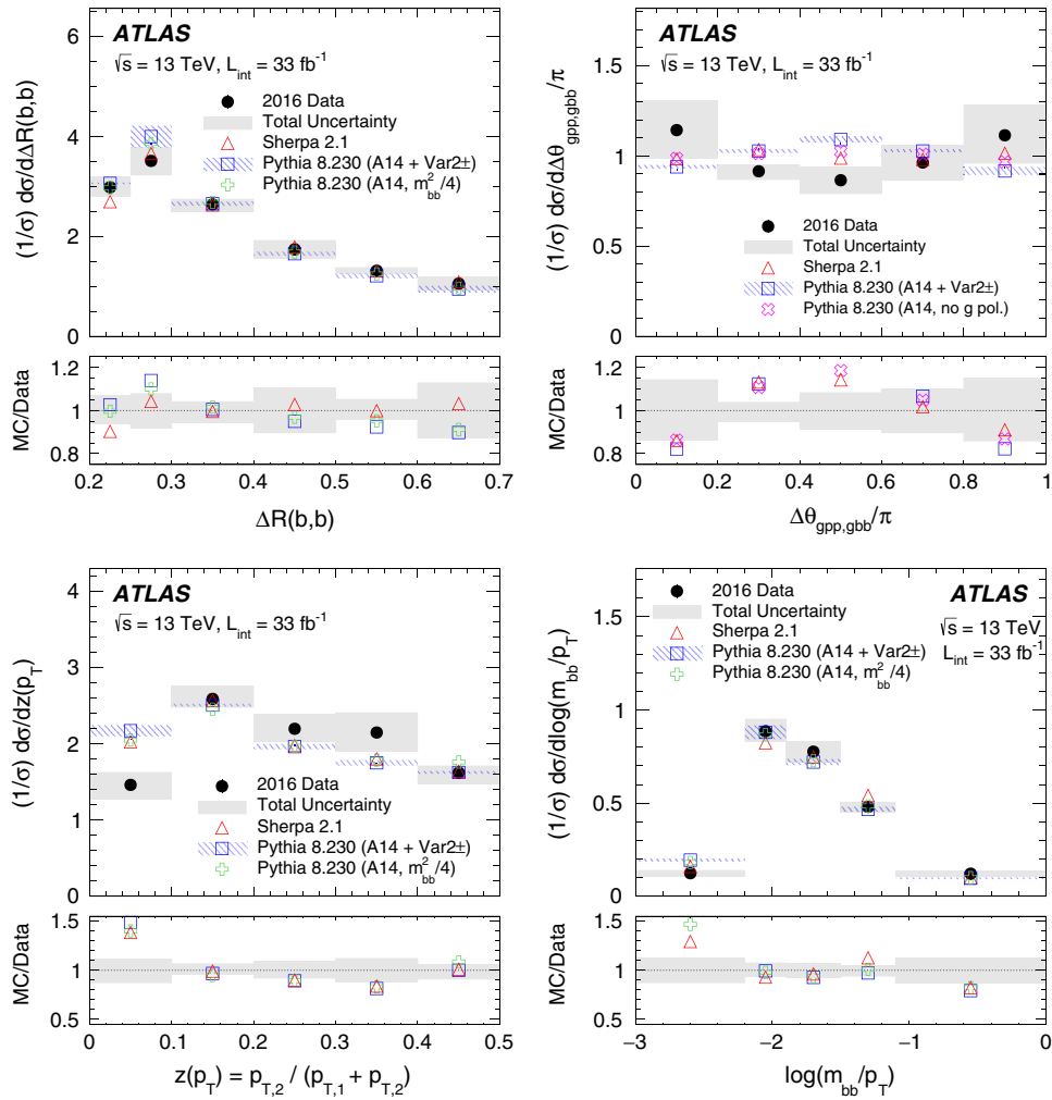
FIG. 6. The unfolded distribution of \Delta R(b, b) (top left), \Delta\theta_{\text{ppg,gb}}/\pi (top right), z(p_T) (bottom left), and \log(m_{bb}/p_T) (bottom right). Error bands represent the sum in quadrature of statistical and systematic uncertainties (see Sec. VIII). These data are compared with predictions from the PYTHIA and SHERPA MC simulations. The bands for the PYTHIA prediction represented by a square indicate the \text{Var}2\pm variations (dominated by a \pm 10\% variation in the final-state shower \alpha_s ). The additional set of PYTHIA markers use m_{bb}^2/4 for the renormalization scale.
