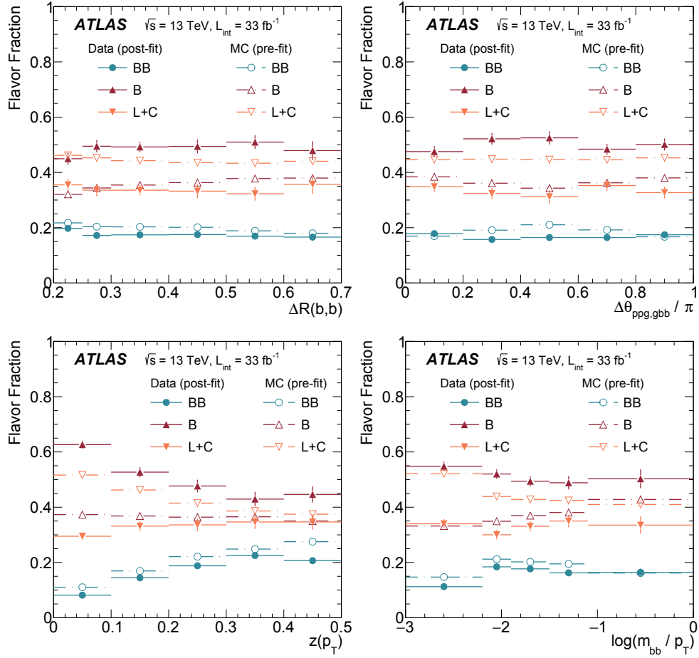
Figure 5: The pre-fit (MC) and post-fit (data) flavor fractions for \Delta R(b, b) (top left), \Delta\theta_{\text{ppg,gb}} (top right), z(p_T) (bottom left), and \log(m_{bb}/p_T) (bottom right) are indicated with open and solid markers respectively. The error bars include only statistical uncertainties from the flavor-fraction fit. The fit's systematic uncertainties are comparable in magnitude, but correlated across the bins. The impact of both the flavor-fraction fit's statistical and systematic uncertainties on the final results is presented in Table 1.
